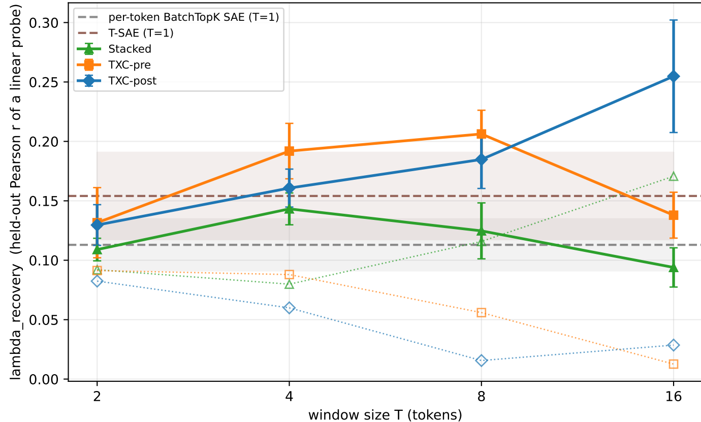
Task hunt Stage 2 — \lambda intensity recovery vs T REAL Ward activations (base, resid_post L12); hollow/dotted = untrained control
