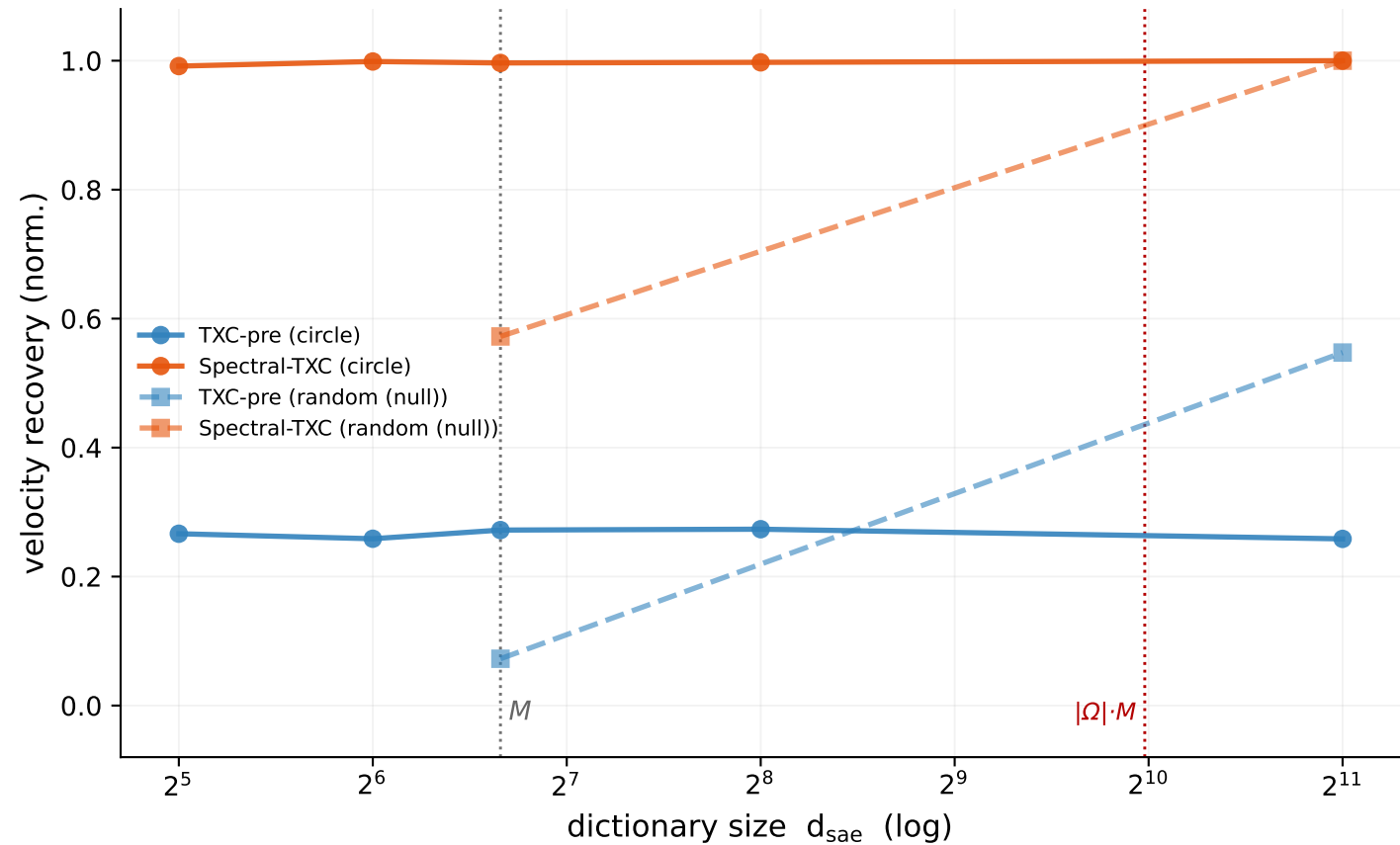
Memorization above |\Omega| \cdot M : the random null jumps to \sim 1 by template lookup
