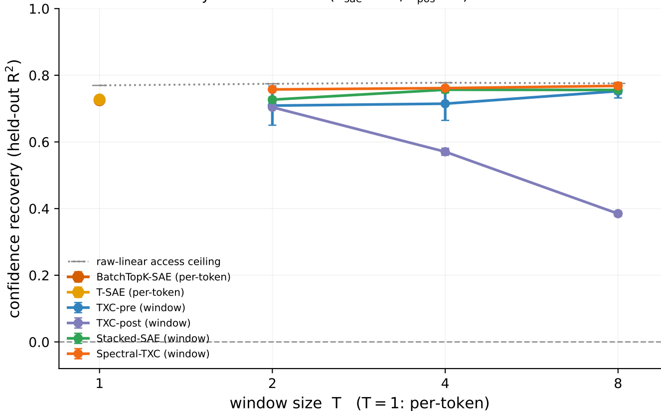
Confidence recovery vs window size ( d_{\text{sae}} = 20 , k_{\text{pos}} = 1 )
