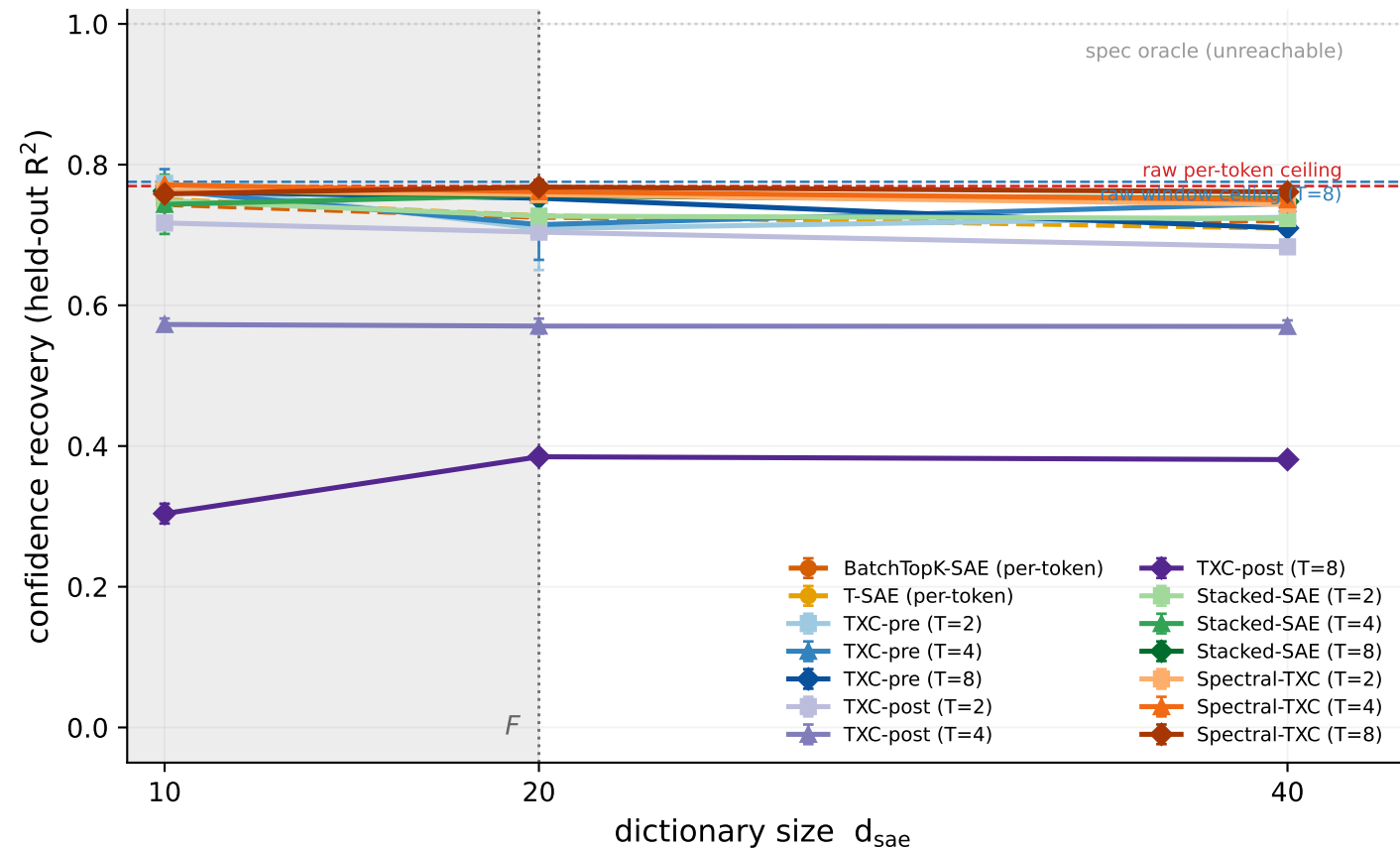
DC latent: confidence state c_i — recovery vs capacity
