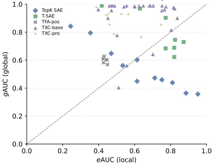
Coupling: dictionary alignment, n_{\text{parents}} = 10
