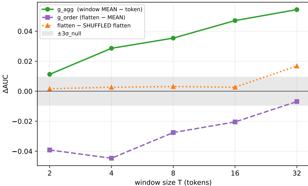
\hat{\lambda}_{\text{hist}} , base L12 — the gap is order-free aggregation
