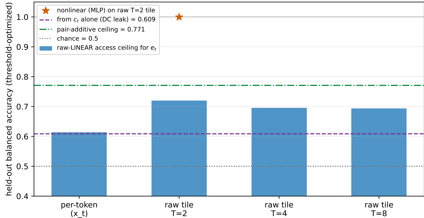
recipe_instruction § 8 equality-variant gate: raw-linear access to e_t vs the analytic DC-leak / additive / nonlinear lines
