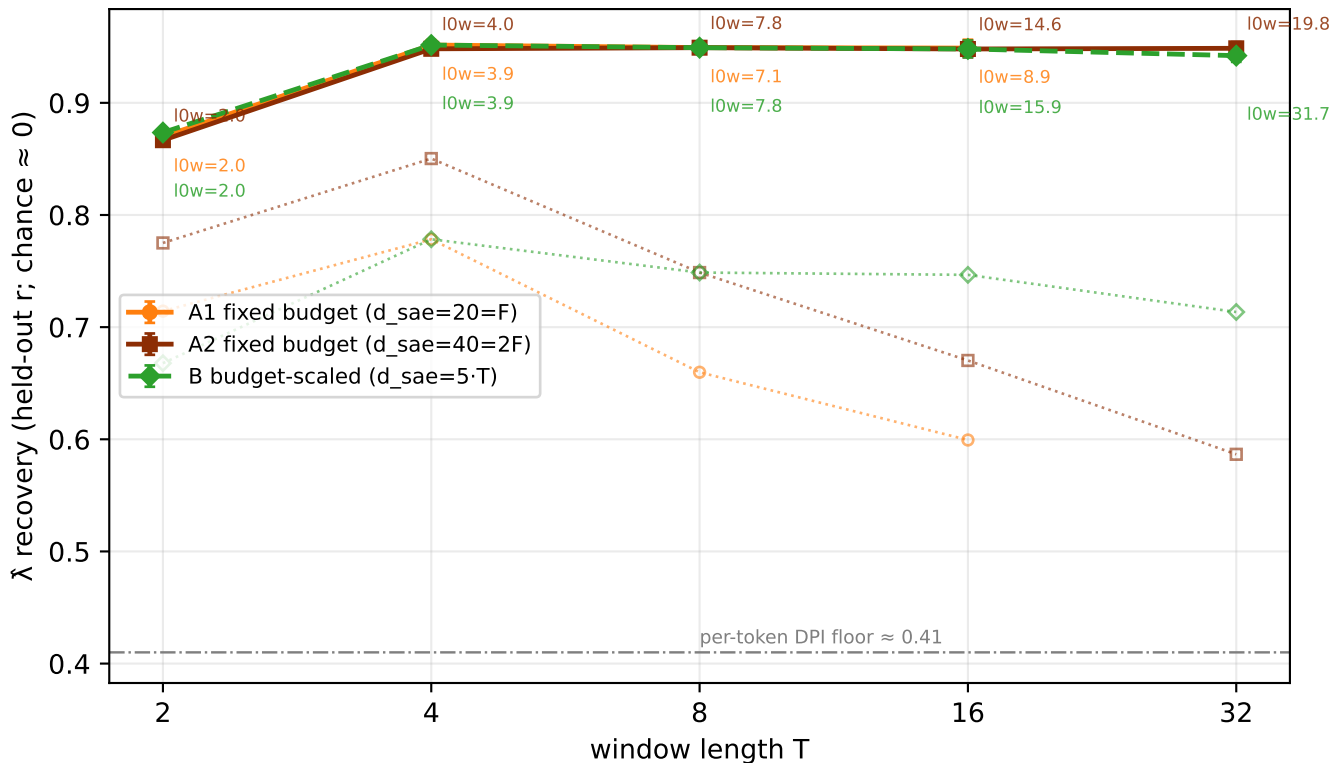
Budget-dilution receipt — TXC-pre, \lambda mirror ( k_{\text{pos}}=1 , L=32 ; solid=trained, dotted=untrained; l0w = realized atoms/window)
