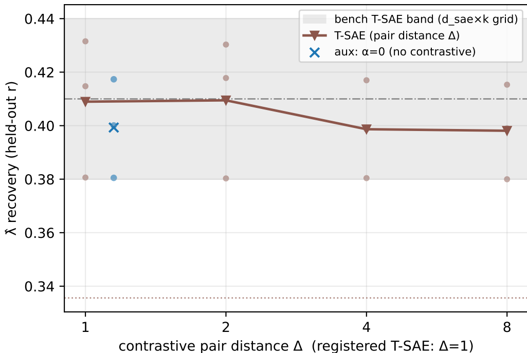
T-SAE fairness receipt — pair-distance knob ( d_{\text{sae}}=20 , k_{\text{pos}}=1 ; dotted = untrained)
