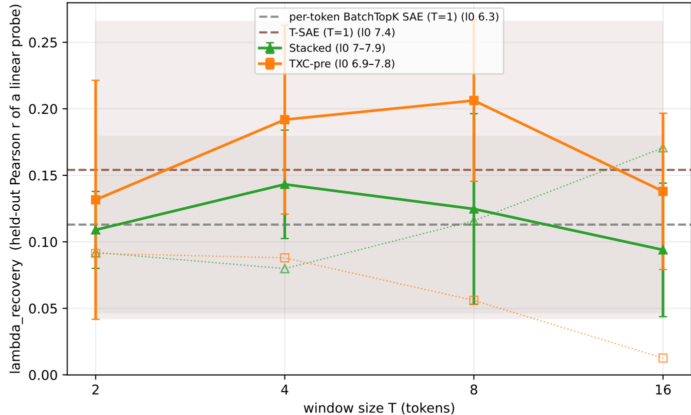
Task hunt Stage 2 — \hat{\lambda} recovery vs T, budget-matched archs only (realized IO within 2× of nominal k; whiskers = 95% t CI over seeds)
