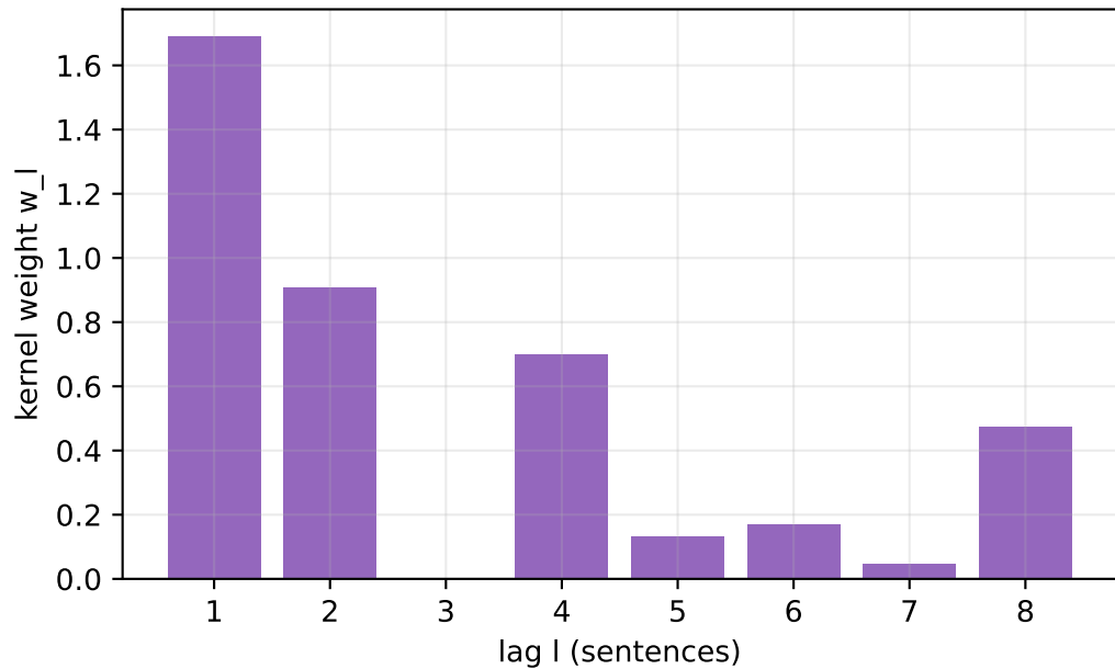
Fitted self-excitation kernel
