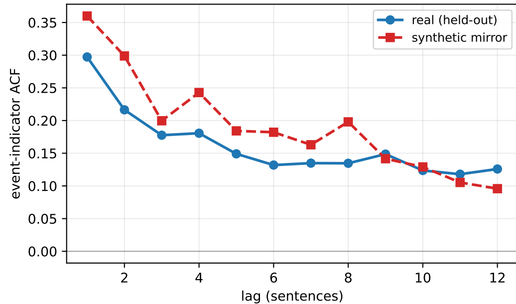
Mirror reproduces the autocorrelation
