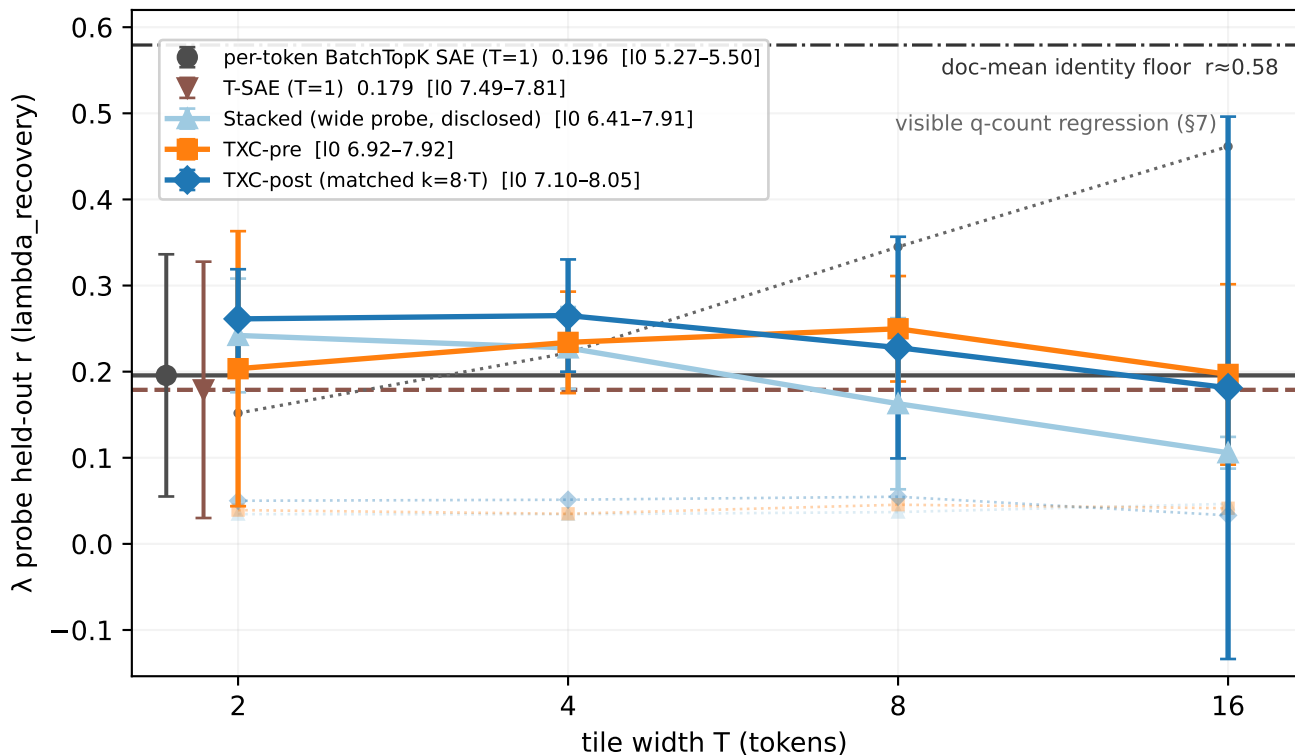
punctint-q fineweb Stage-2 panel — gemma-2-2b hs14 (v1, canonical)
