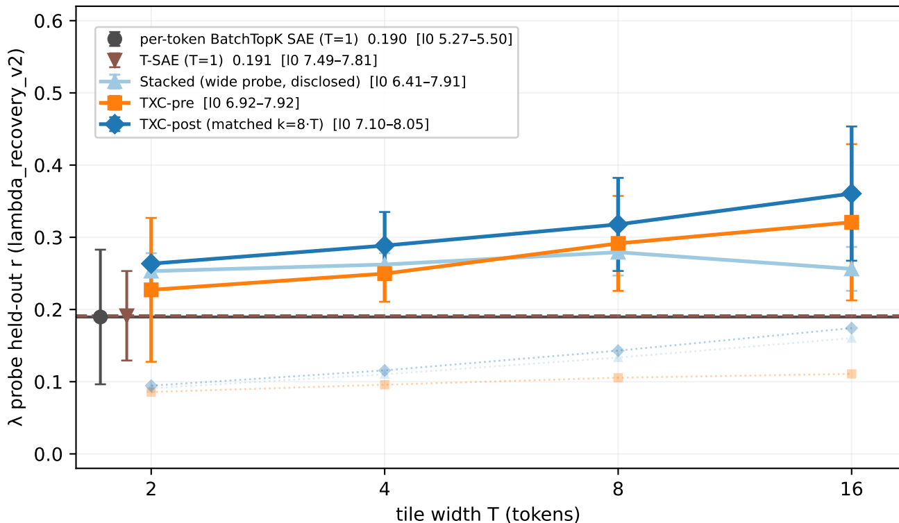
punctint-q fineweb Stage-2 panel — gemma-2-2b hs14 (paired v2 — not canonical)
