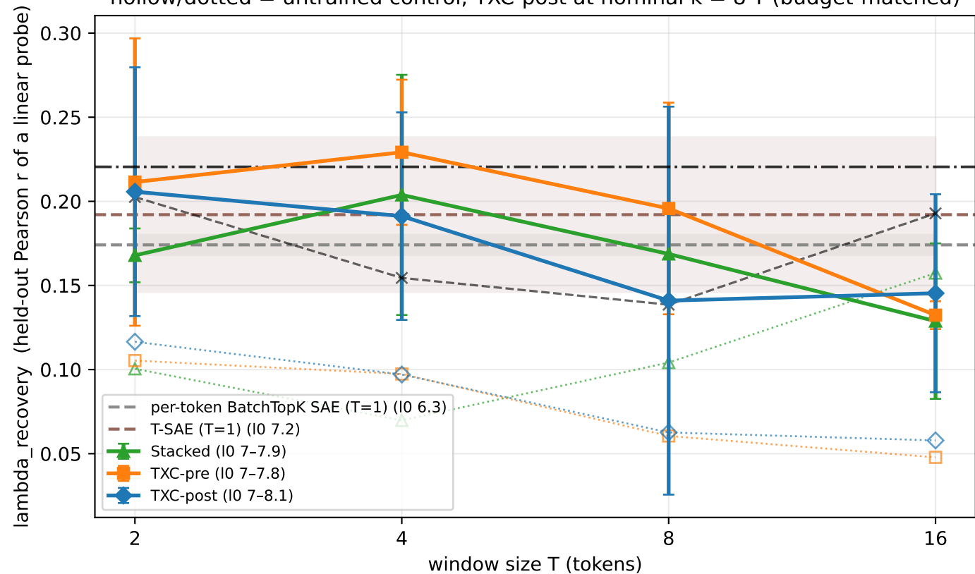
Task hunt Stage 2 — hedging-trend (slope8) recovery vs T REAL Ward activations (R1-Distill, resid_post L14); whiskers = 95% t CI over seeds; hollow/dotted = untrained control; TXC-post at nominal k = 8·T (budget-matched)
