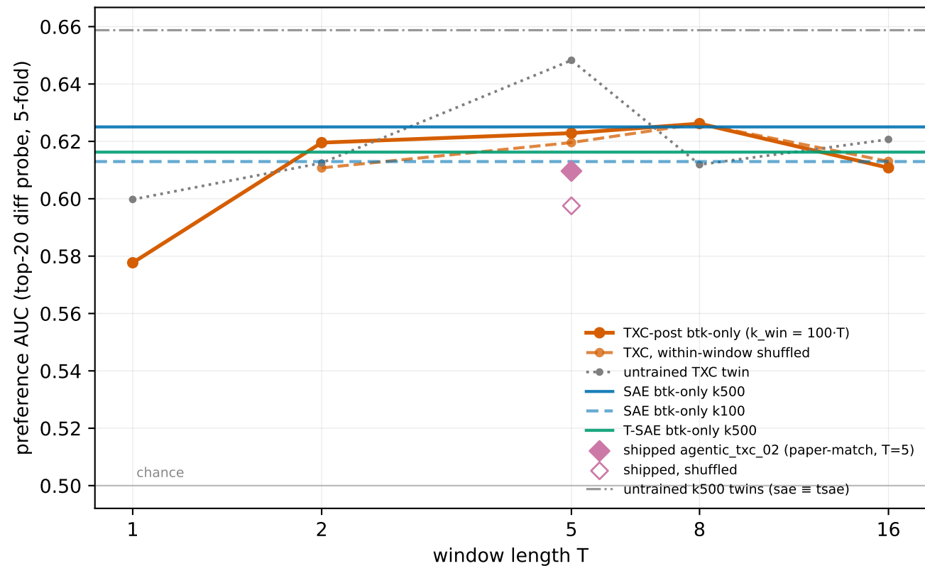
HH-RLHF § 5.4 — btk-only T-sweep + the missing shuffle control (seed 42)
