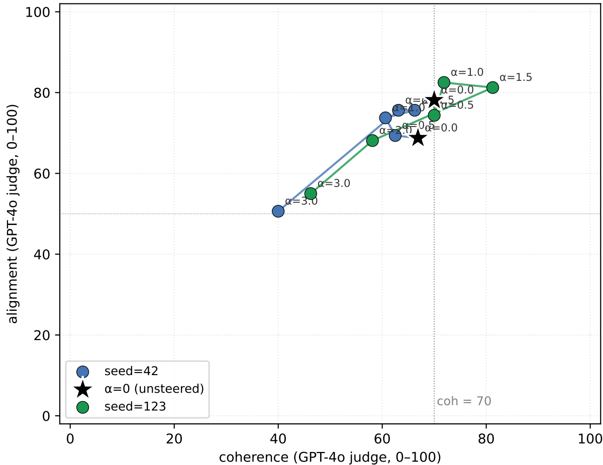
SAE-resid steering @ blocks.25.ln1.hook_normalized (medical EM, k=64, top-50 features)
