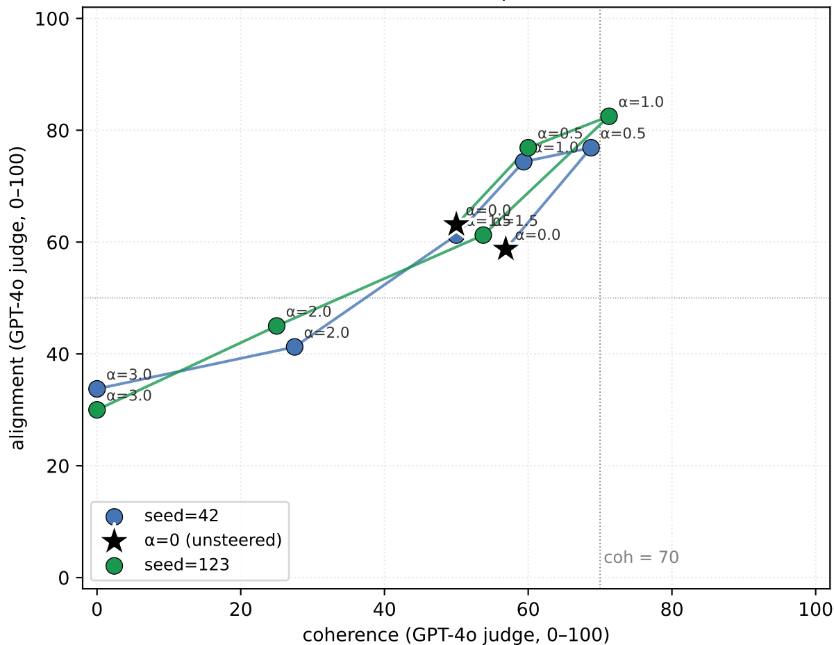
SAE-resid steering @ blocks.24.hook_resid_mid (medical EM, k=64, top-50 features)
