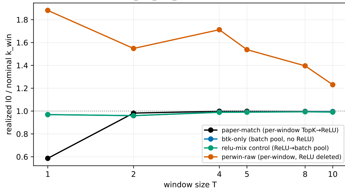
coupled_K10_M20_d256 — mixing fingerprint
