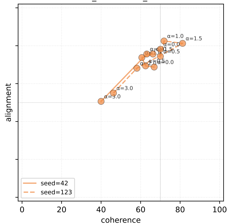
ln1_normalised_L25
