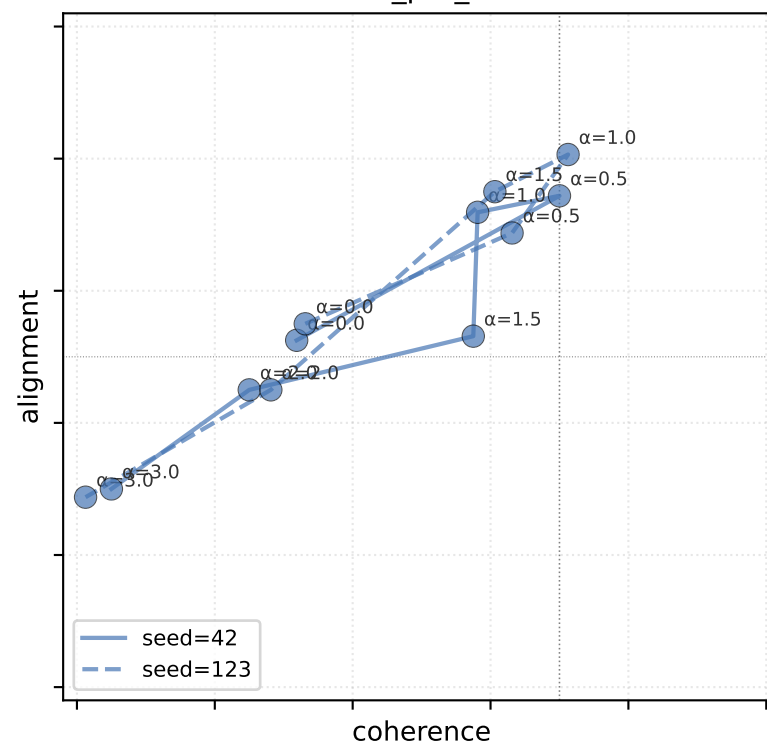
ln1_normalised_L25
