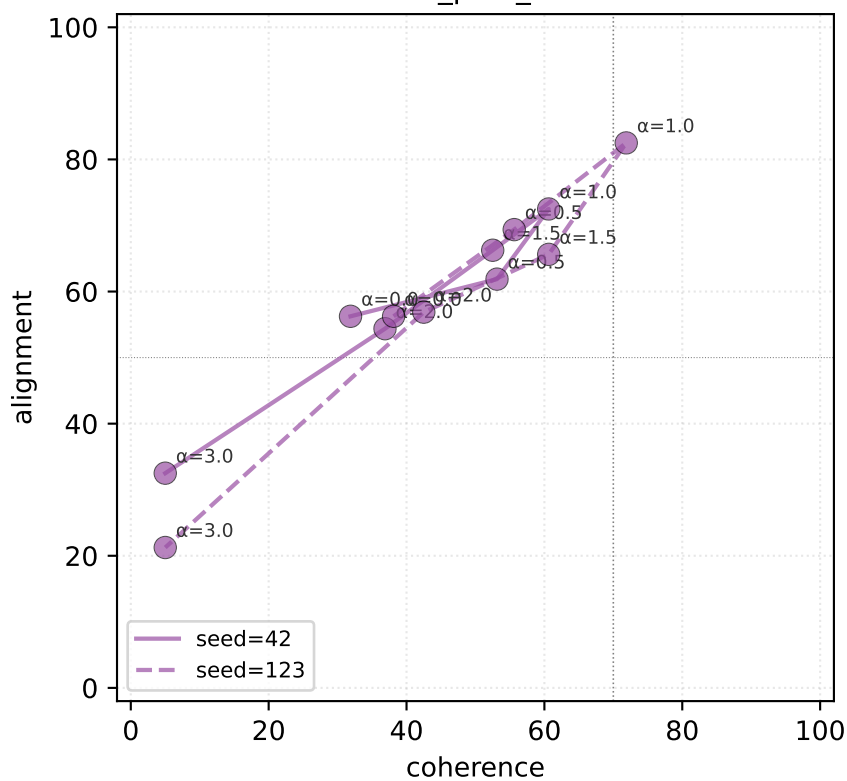
resid_post_L24
