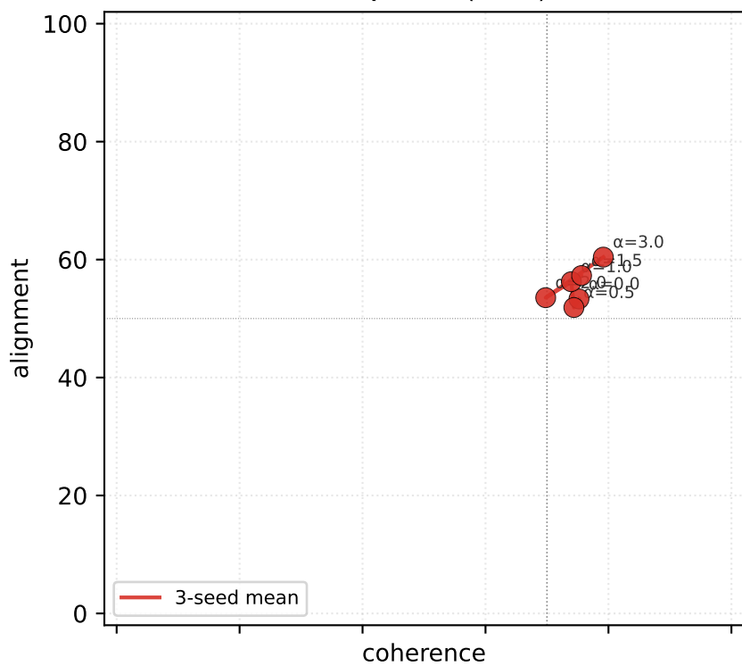
resid_post_L24
