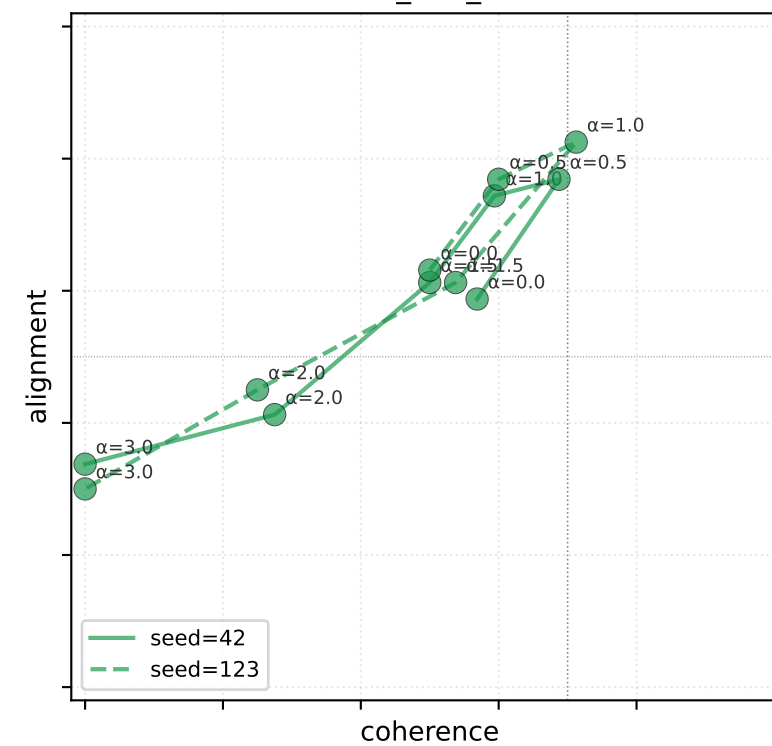
resid_mid_L24
