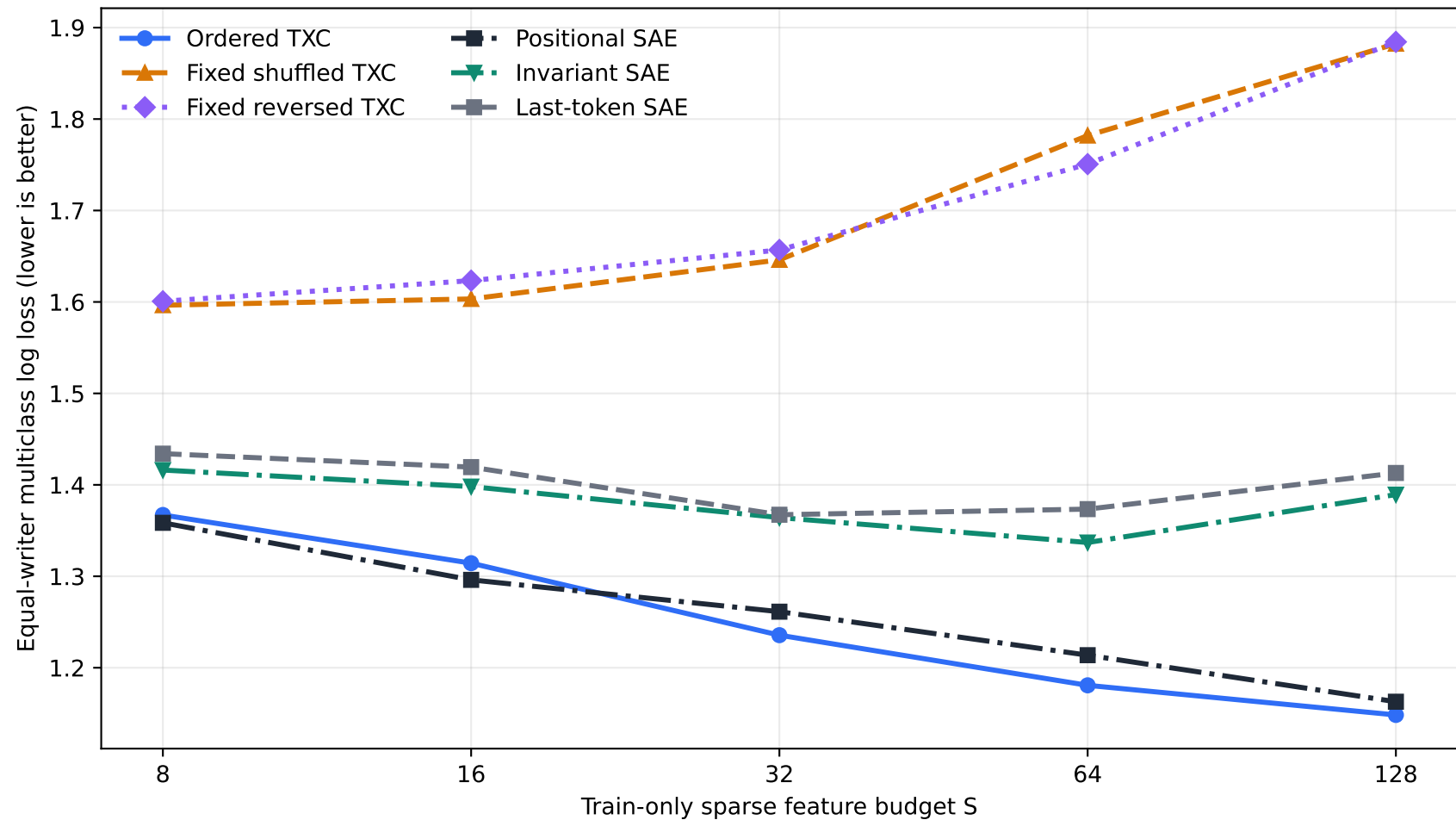
Frozen T=5 dictionaries on human deletion destination
