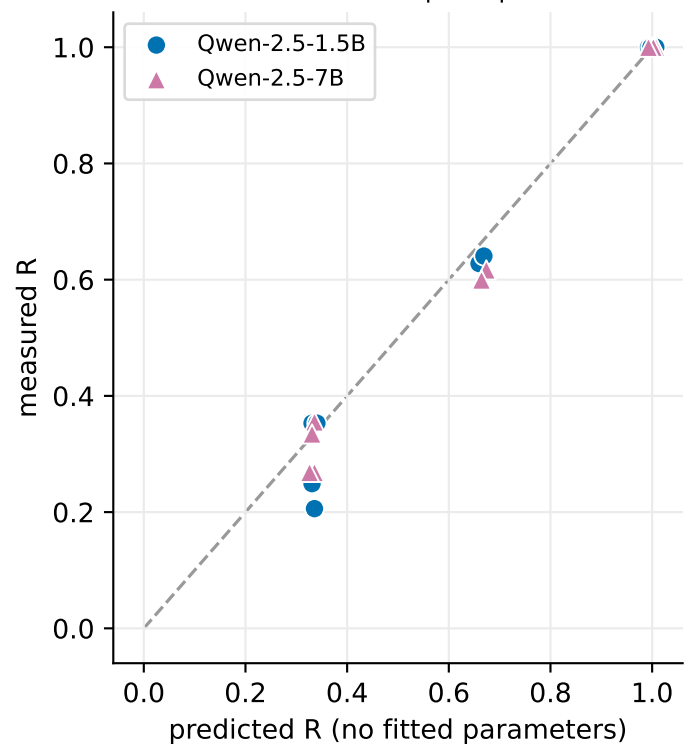
C. Same law in both models 6 fractional cells: mean |error| 0.053 / 0.045
