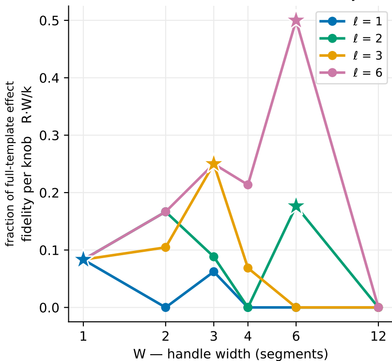
B. Control efficiency peaks at W \approx \ell (★ = best width; knobs needed for full fidelity = k/\ell )
