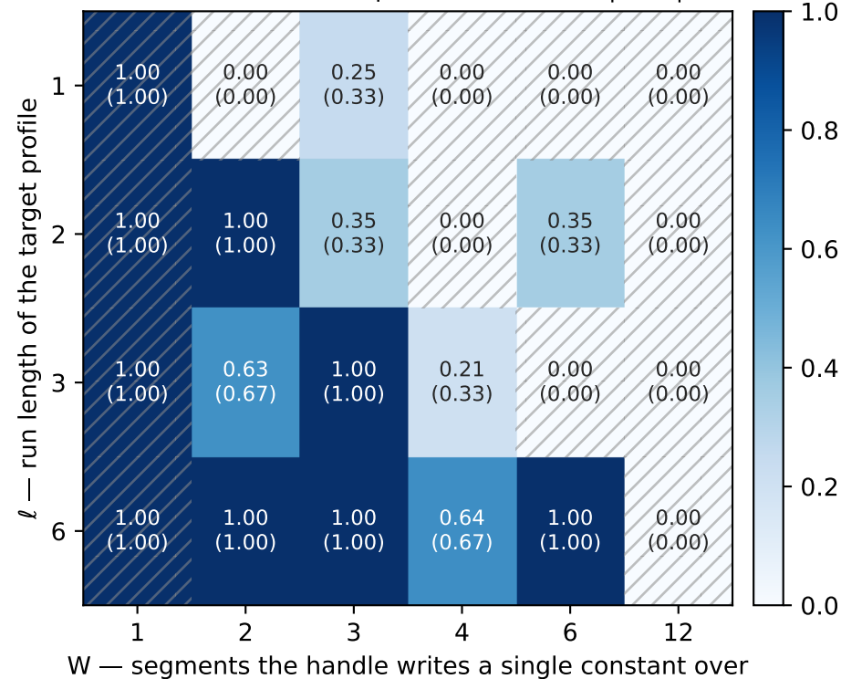
A. Fidelity R(W, \ell) : observed, (predicted) 11 measured cells, no fitted parameters, mean |error| = 0.029
