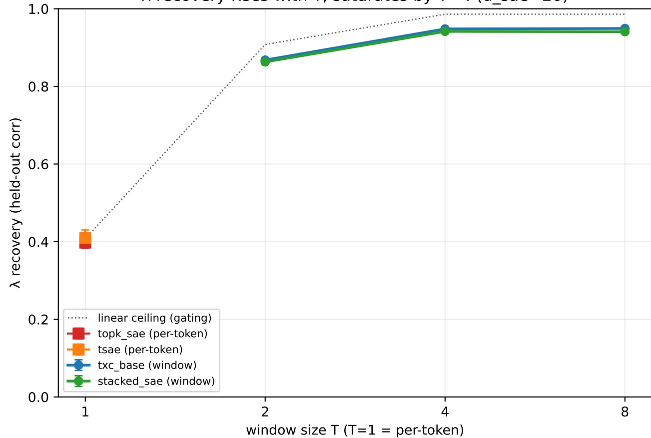
\lambda recovery rises with T, saturates by T=4 (d_sae=20)
