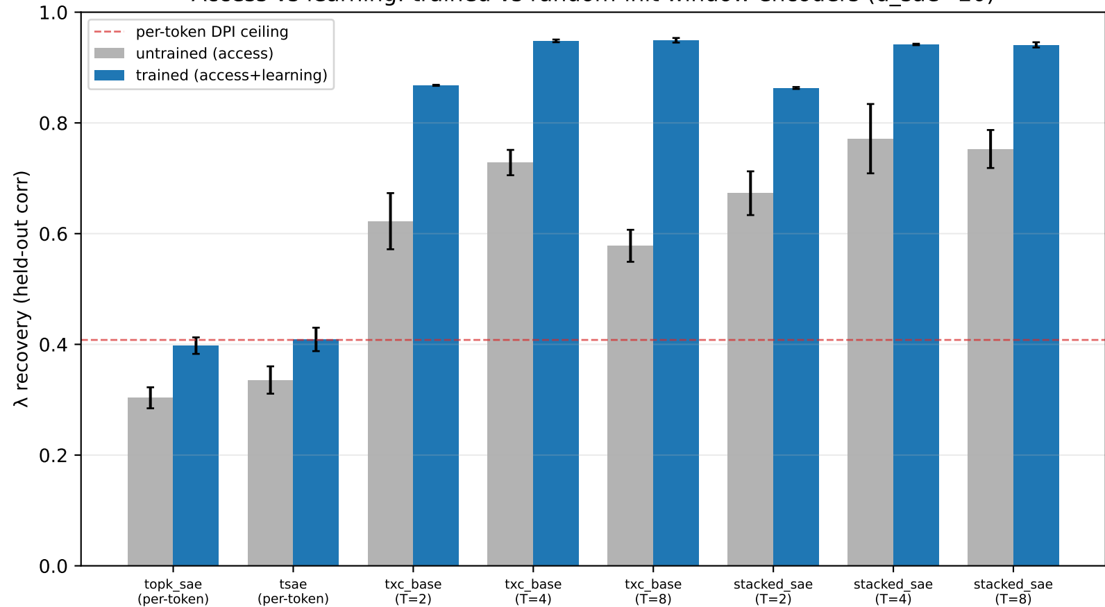
Access vs learning: trained vs random-init window encoders (d_sae=20)
