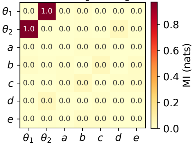
(C) Cubic: \theta_1 = (10\theta_2)^3
