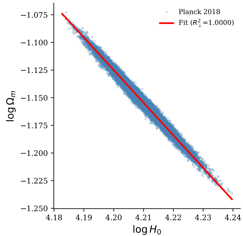
(a) Planck 2018: \Omega_m h^3 \approx \text{const} degeneracy
