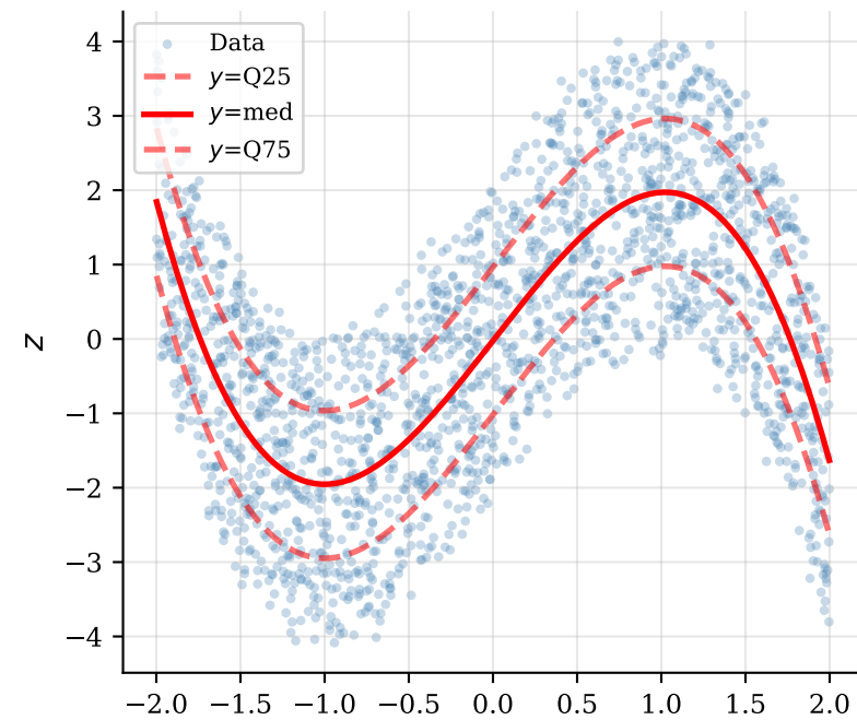
Cubic: \theta_1 - (10\theta_2)^3 \approx 0
