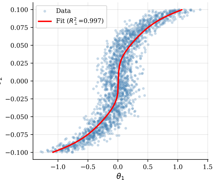
Cubic: \theta_1 - (10\theta_2)^3 \approx 0
