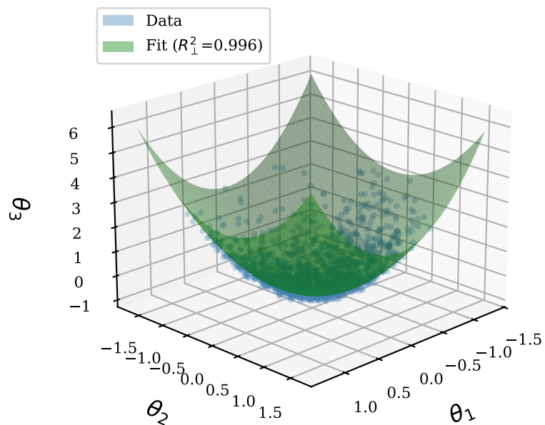
Banana: 2\theta_1^2 + \theta_2^2 - \theta_3 = 0.5
