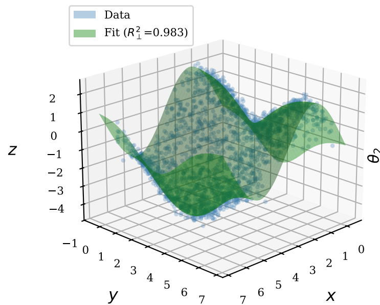
Trig: 2\sin(x) + \cos(y) - z = 1
