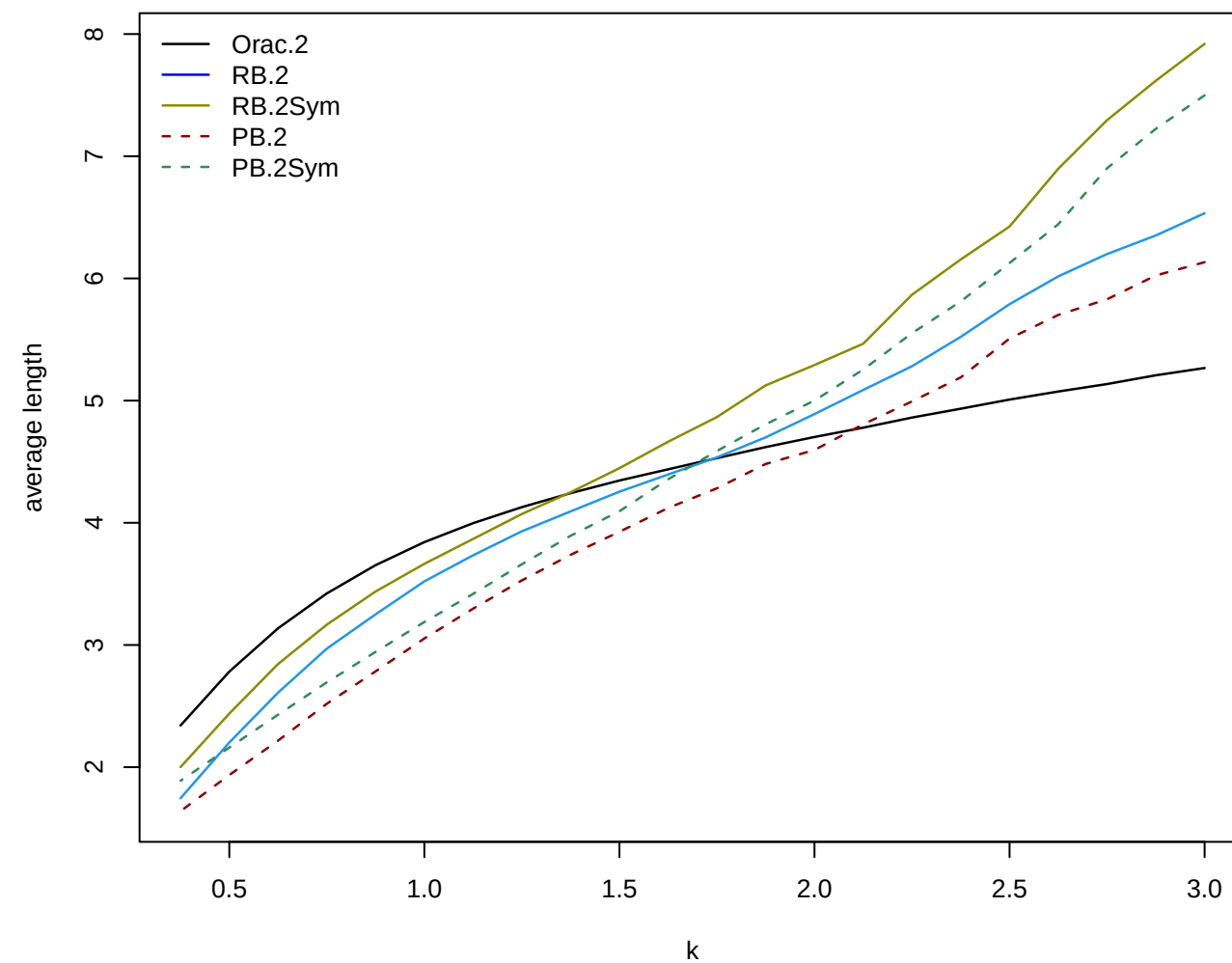
average length of 90% two-sided CIs: homoskedastic case
