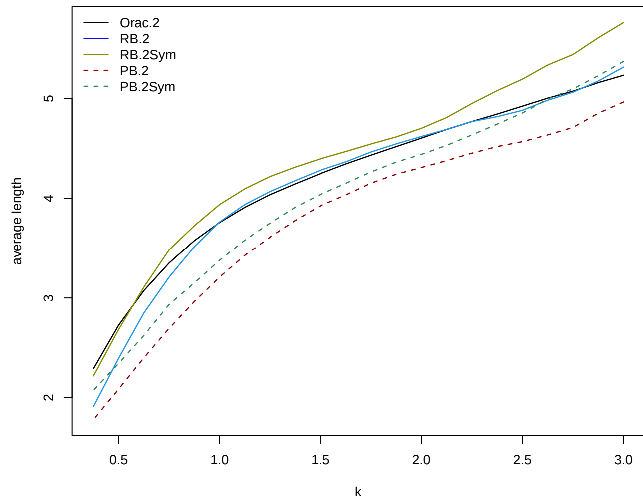
average length of 90% two-sided CIs: homoskedastic case
