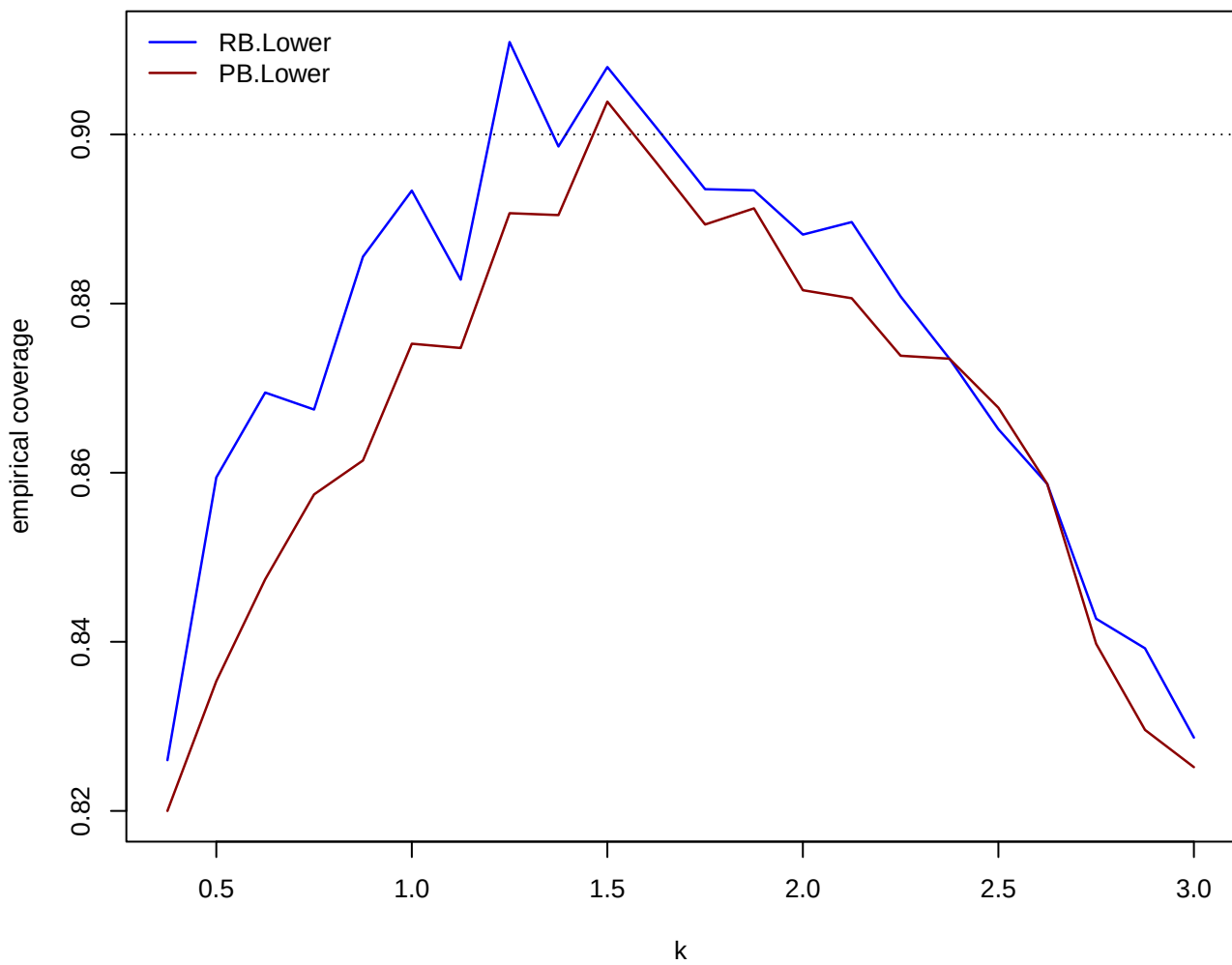
empirical coverage of 90% one-sided lower CIs: homoskedastic case
