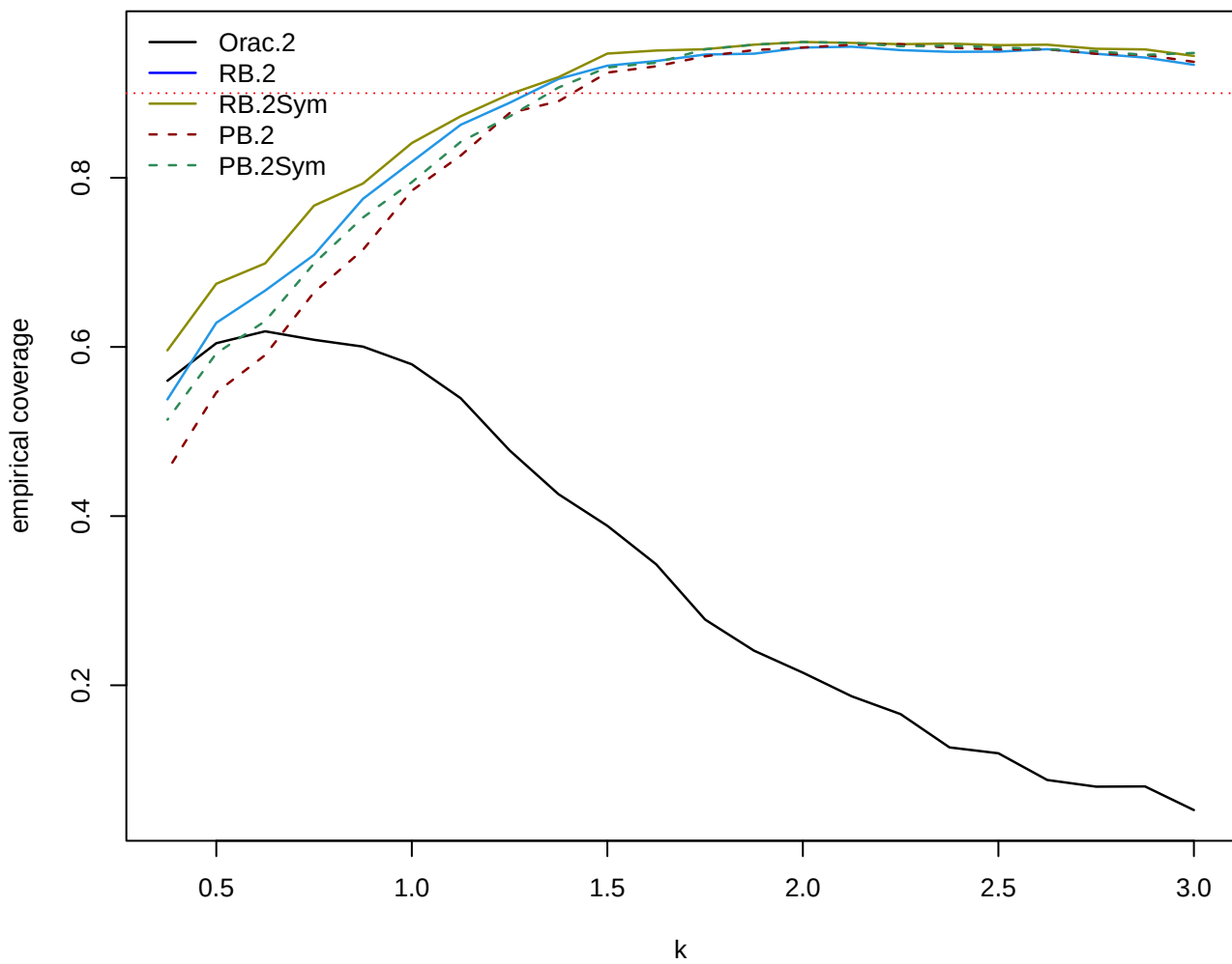
empirical coverage of 90% two-sided CIs: homoskedastic case
