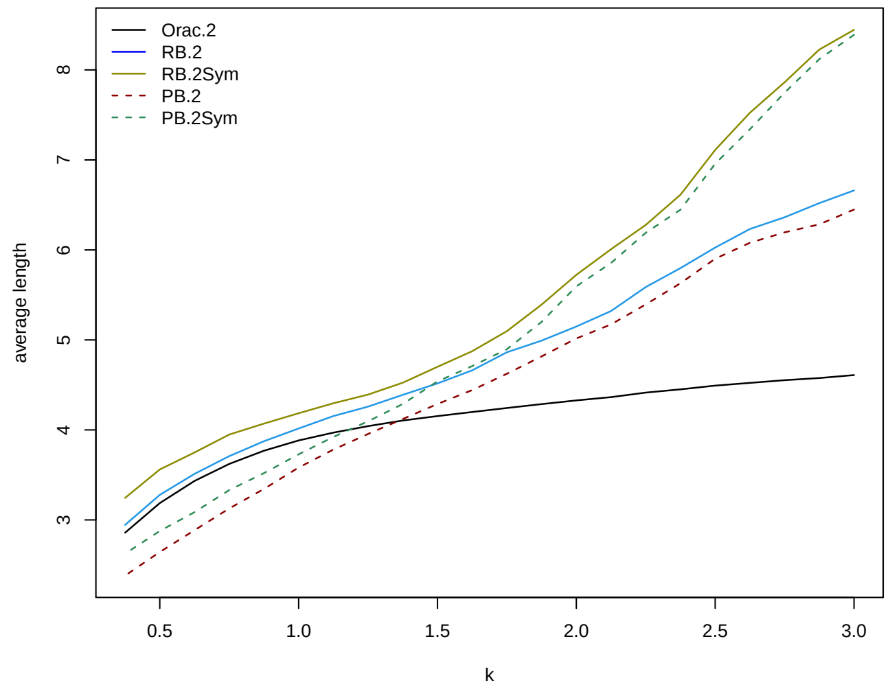
average length of 90% two-sided CIs: homoskedastic case
