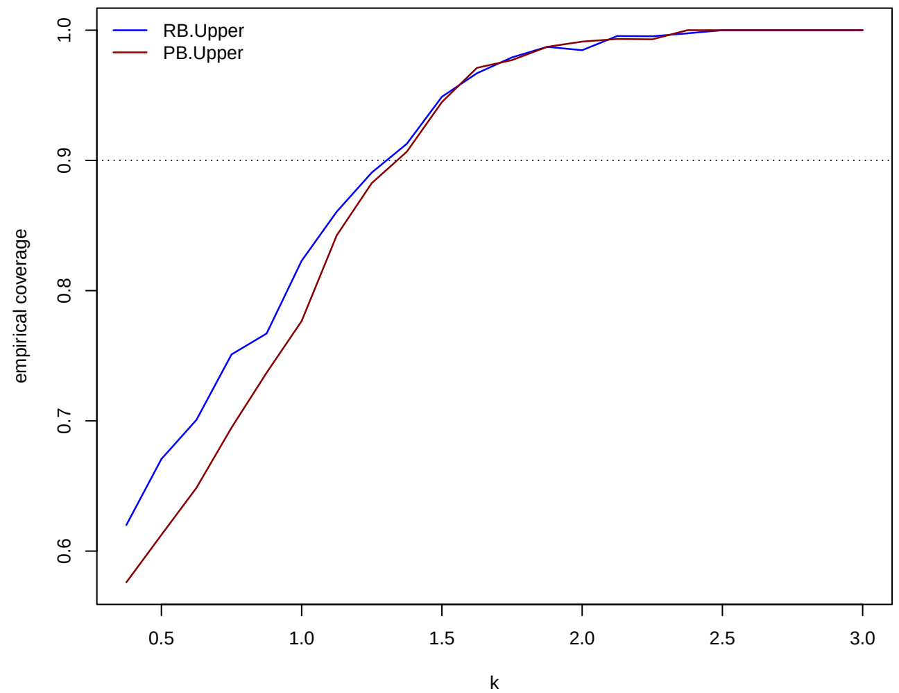
empirical coverage of 90% one-sided upper CIs: homoskedastic case
