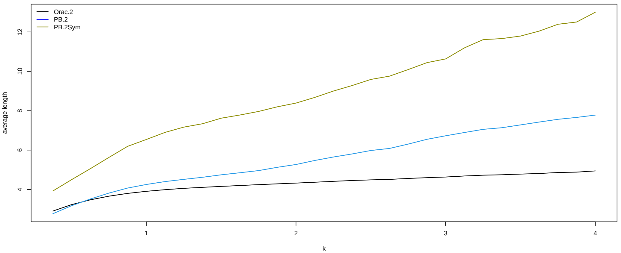
average length of 90% two-sided CIs: heteroskedastic case
