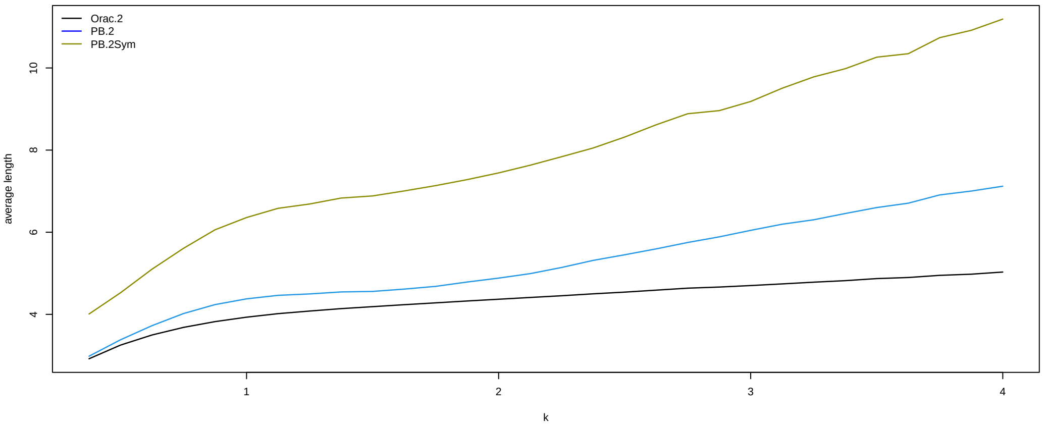
average length of 90% two-sided CIs: heteroskedastic case
