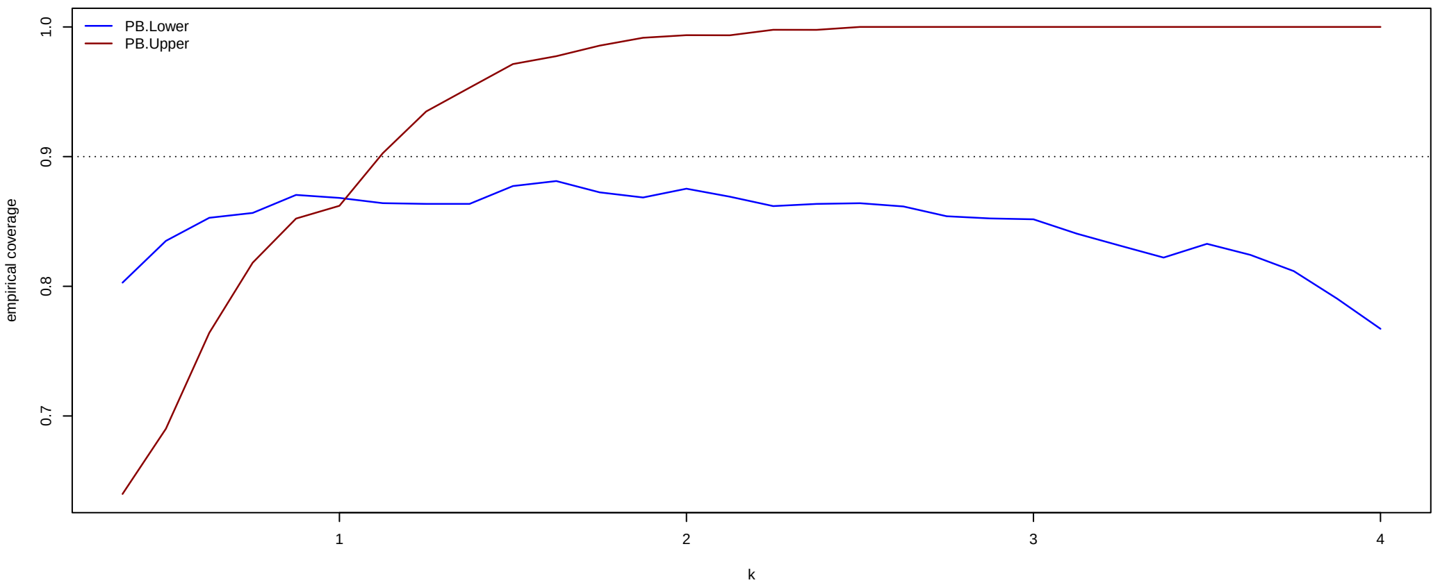
empirical coverage of 90% one-sided lower and upper PB based CIs': heteroskedastic case
