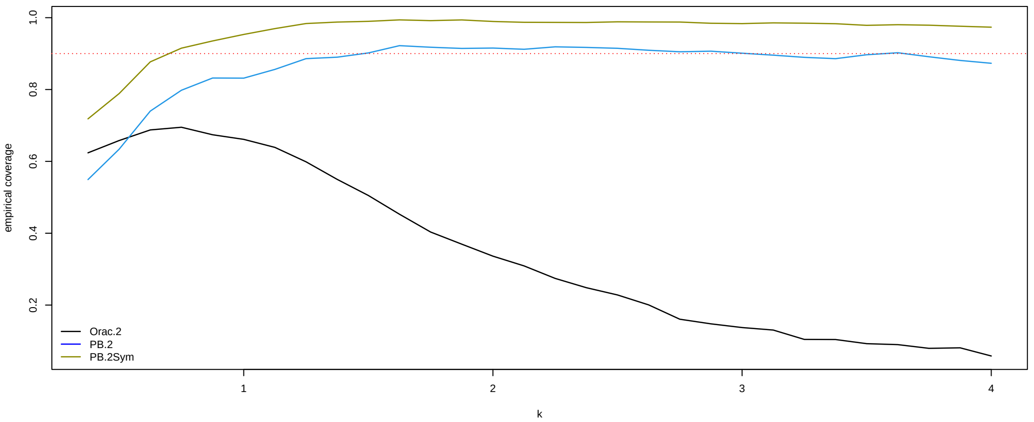
empirical coverage of 90% two-sided CIs: heteroskedastic case
