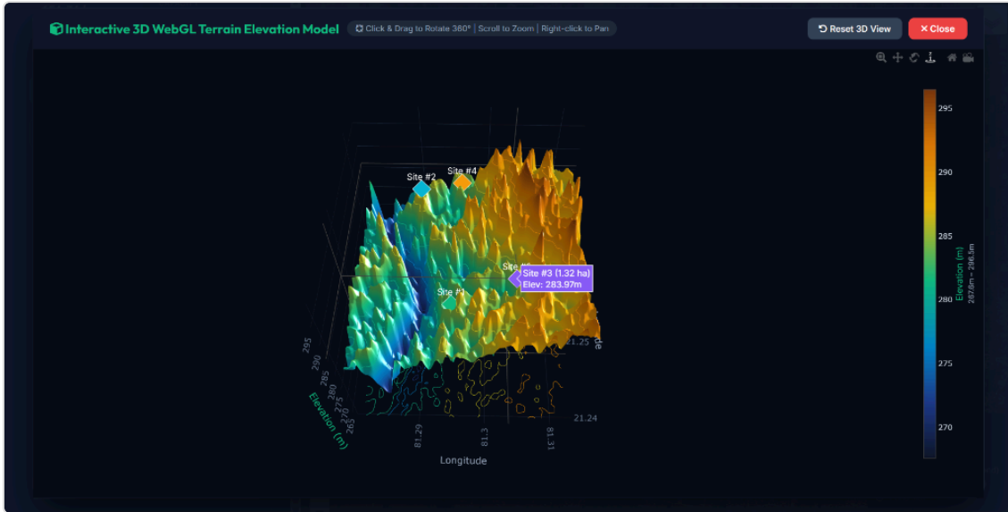
Figure 3: Interactive 3D WebGL Terrain Elevation Model rendered via Plotly.js, displaying topography relief, candidate pond pins (#1–#4), and 2D contour projections.
