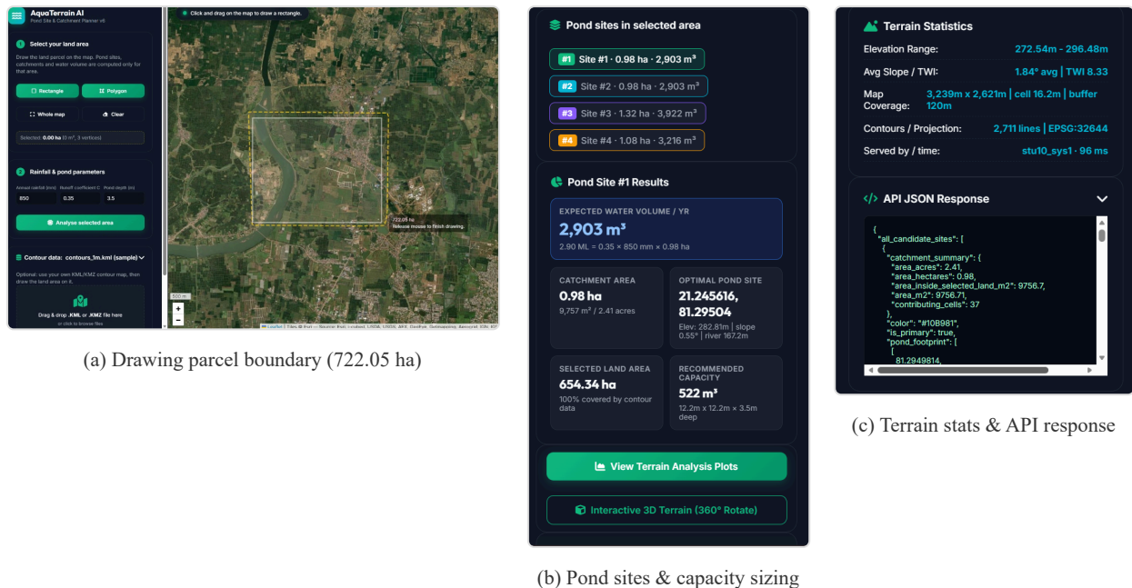
Figure 2: End-to-end interactive workflow: (a) Drawing agricultural land parcel on map; (b) Ranked candidate pond sites and sizing recommendation; (c) Terrain summary statistics and structured JSON API payload served by stu10_sys1 .
