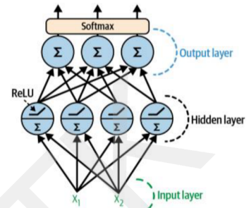
A modern MLP (including ReLU and softmax) for classification.
