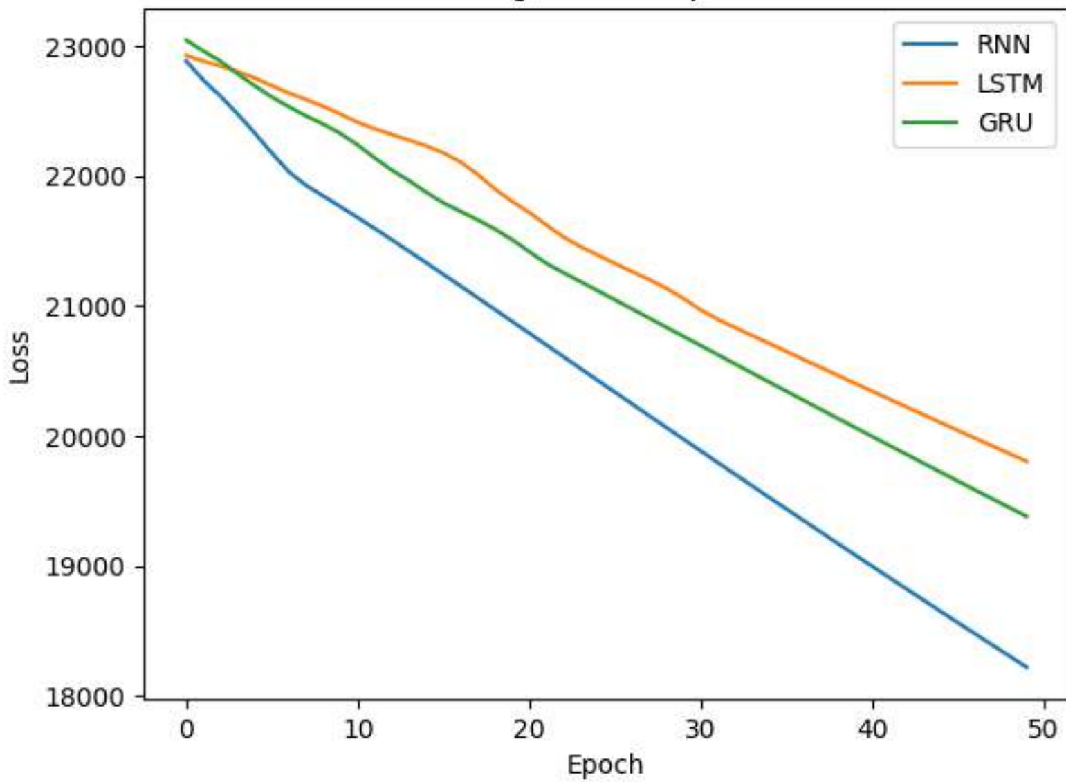
Training Loss Comparison
