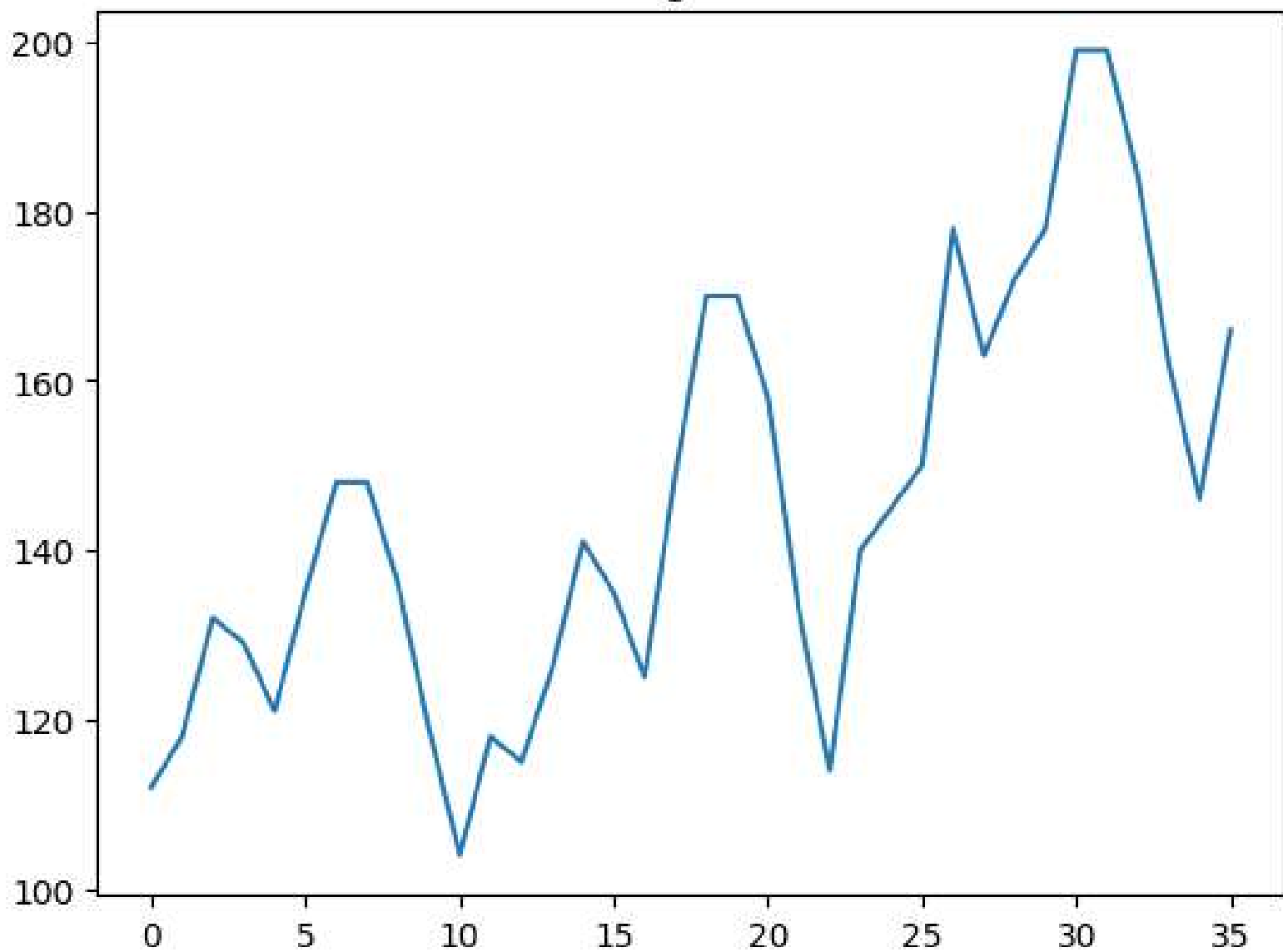
Airline Passengers Time Series
