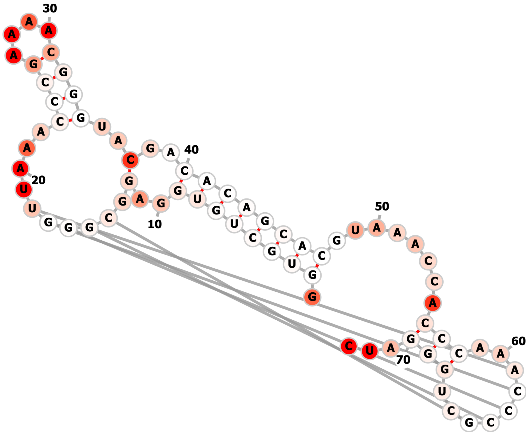
ZMP Riboswitch: Best gRNAde Design (Score = 94.3)
