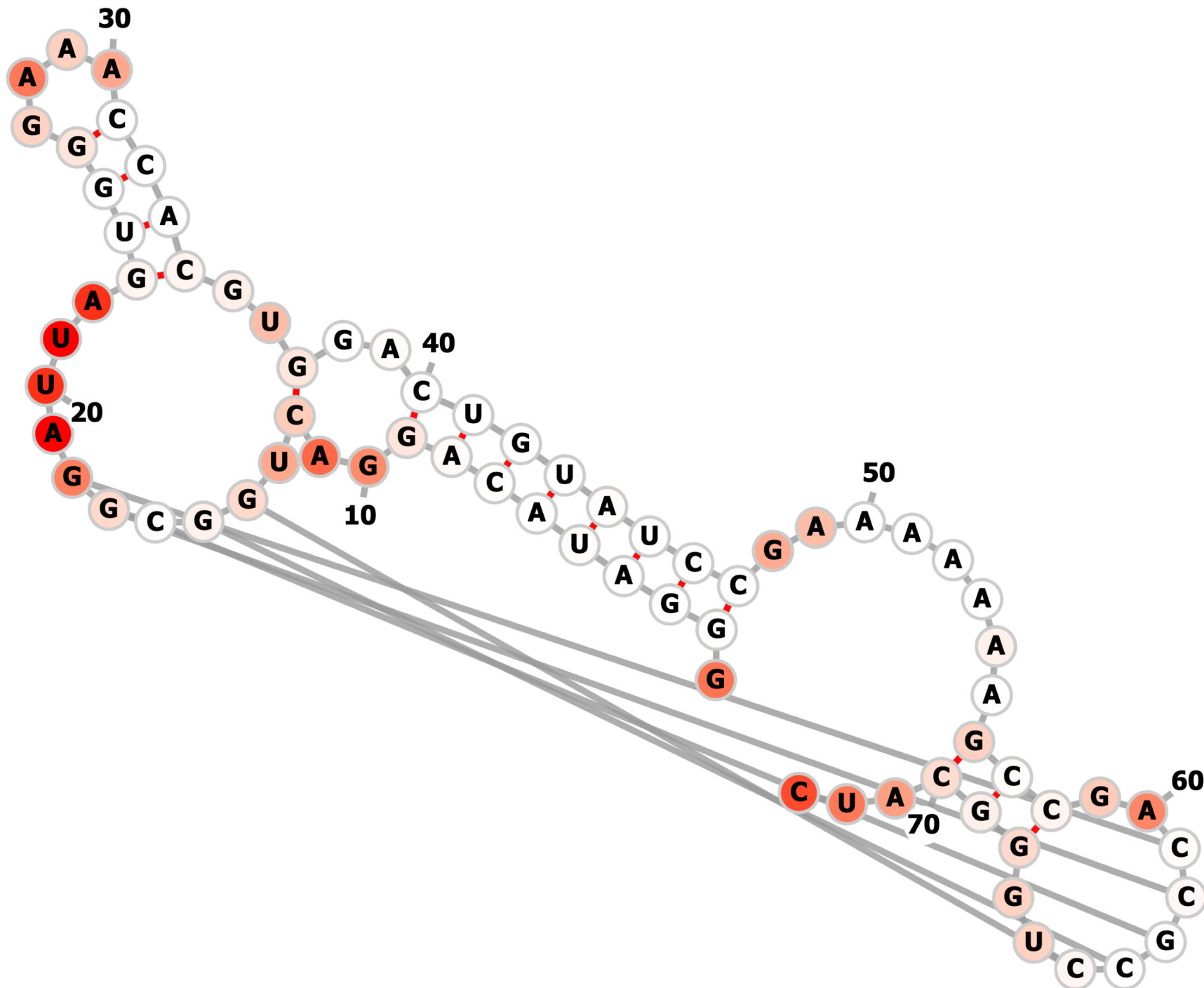
ZMP Riboswitch: WT Sequence (Score = 90.0)
