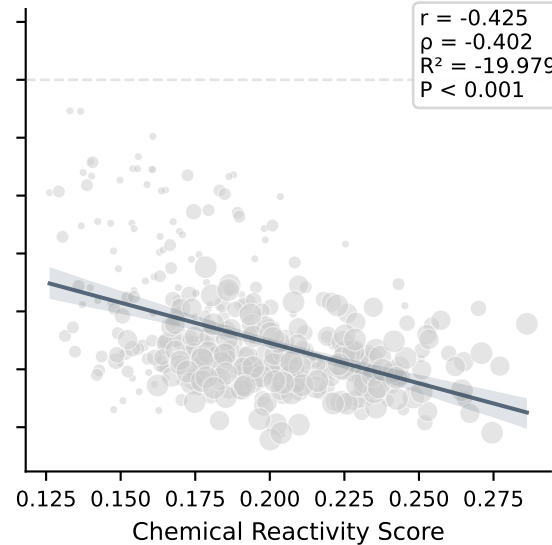
Only rational design (n = 440)
