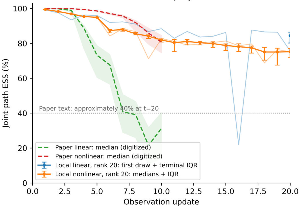
Predator-prey
