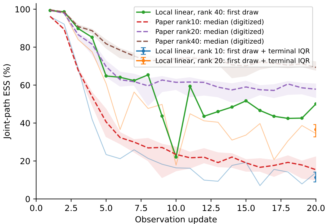
SIR, 18 states
