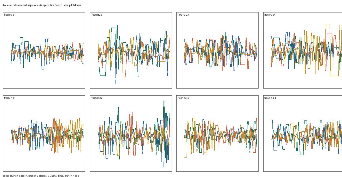
Figure 50.1: Four-launch trajectories in transformed coordinates for the first 64 retained, confirmation-excluded pilot draws of each G and H chain. Colors identify launches. Overlap is an initialization-robustness diagnostic only; neither arm is a posterior oracle.
