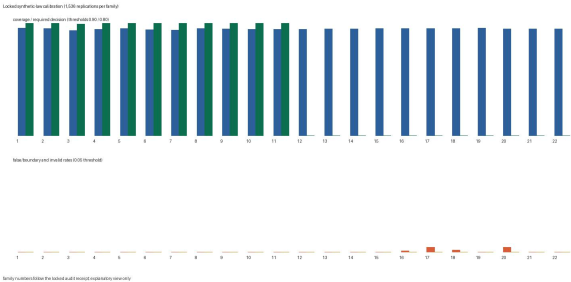
Figure 50.5: Operating characteristics from the locked synthetic-law audit. Blue and green bars are empirical coverage and required-decision rates; orange and gold bars are false/boundary and invalid rates. Family numbers follow the immutable audit receipt. This figure concerns controlled-law calibration, not the G/H retained posterior.
