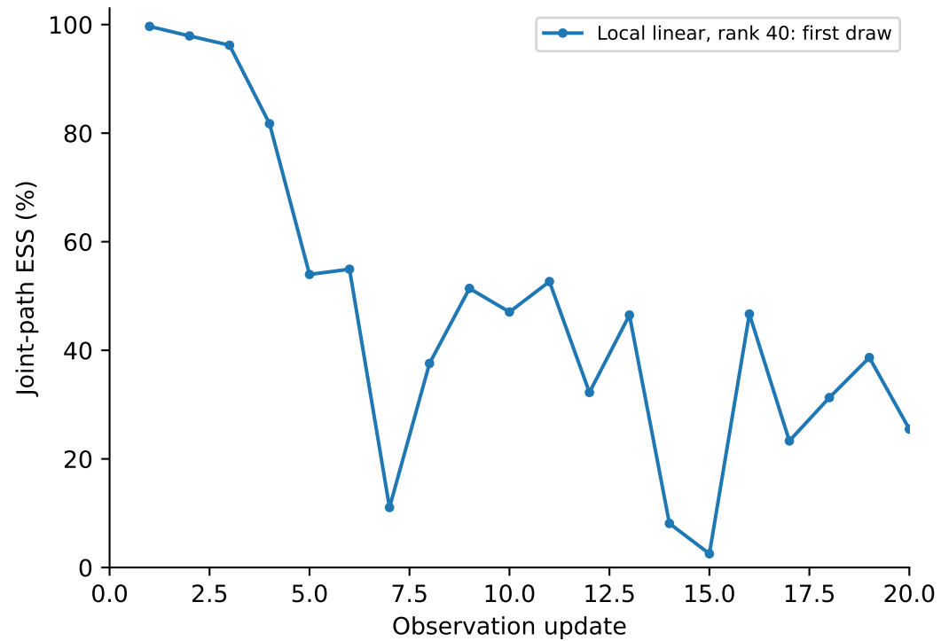
SIR, 18 states
