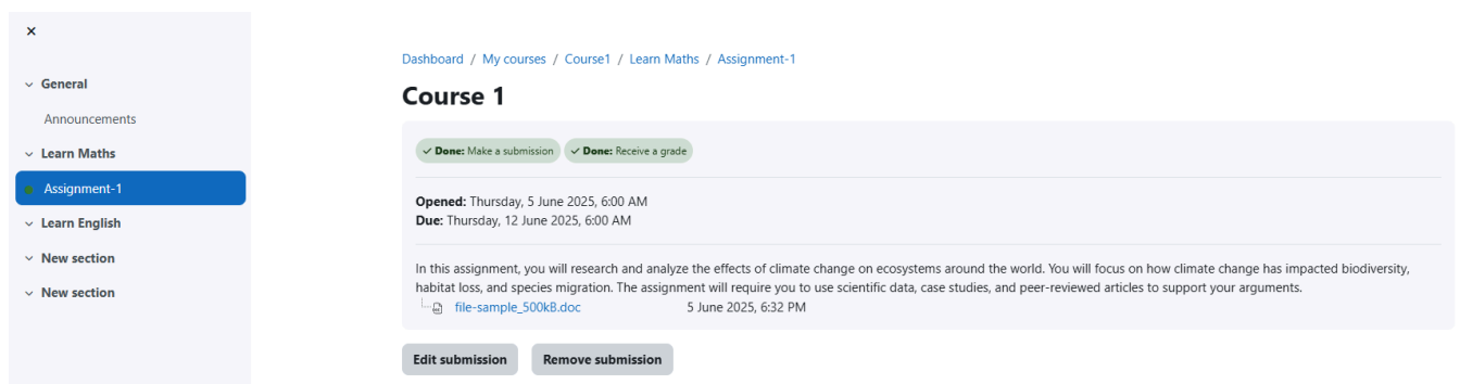
Figure 21. Assignment section
