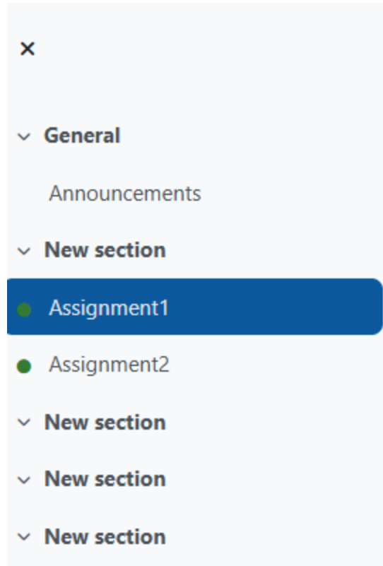
Figure 20. Course sections
