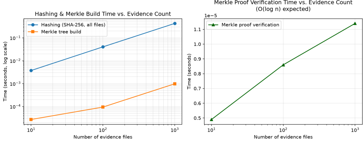
Fig. 1. Hashing and Merkle-tree build time (log-log, left) and Merkle proof verification time (right) versus evidence-file count.
