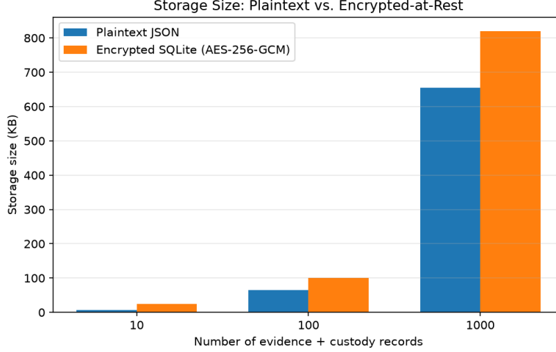
Fig. 2. Plaintext JSON size versus encrypted (AES-256-GCM) SQLite size, by record count.
