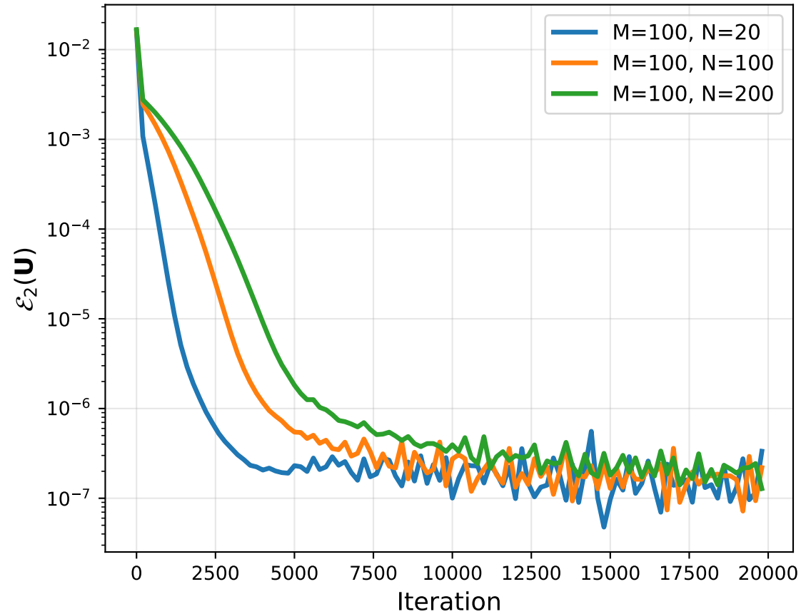
Validation L2 error decay
