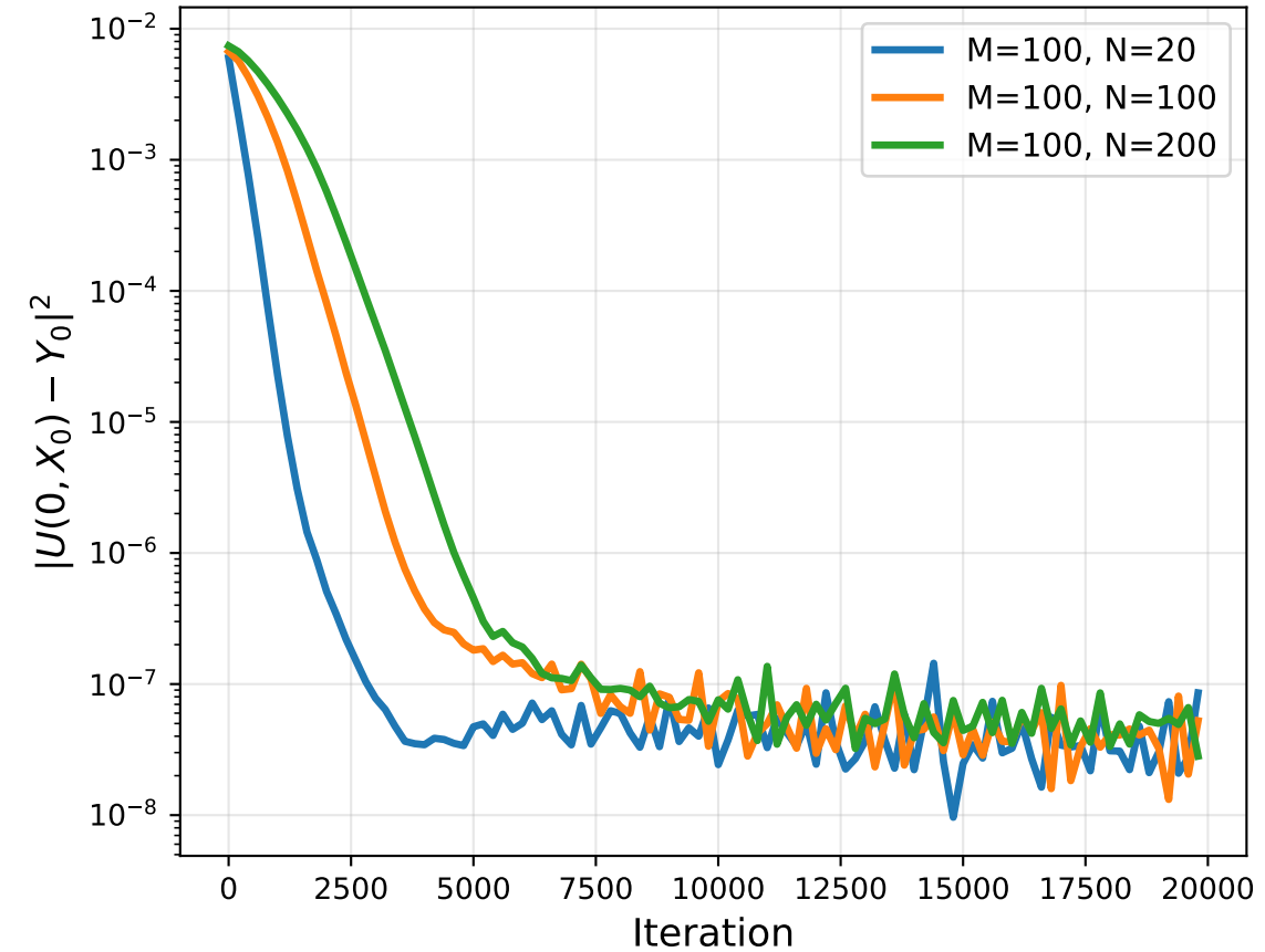
Initial value error decay
