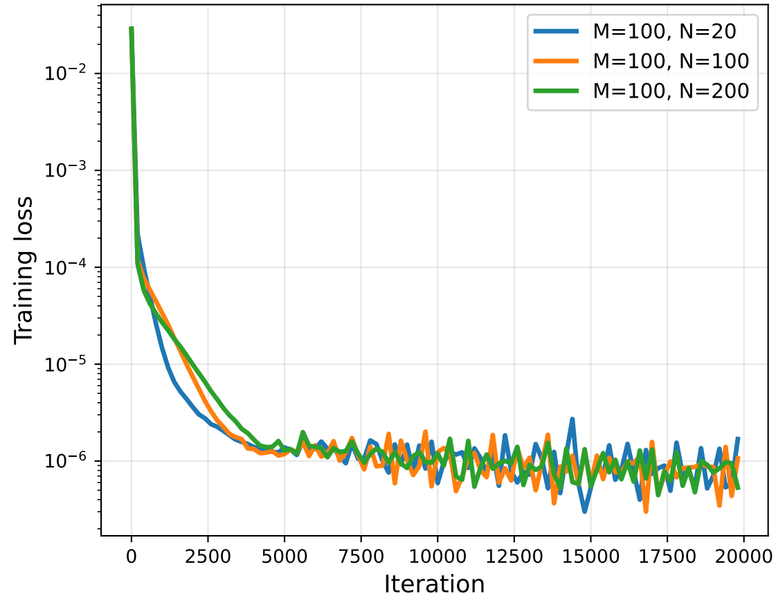
Training loss decay
