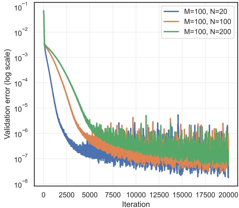
L2 Error decay for different (M, N)
