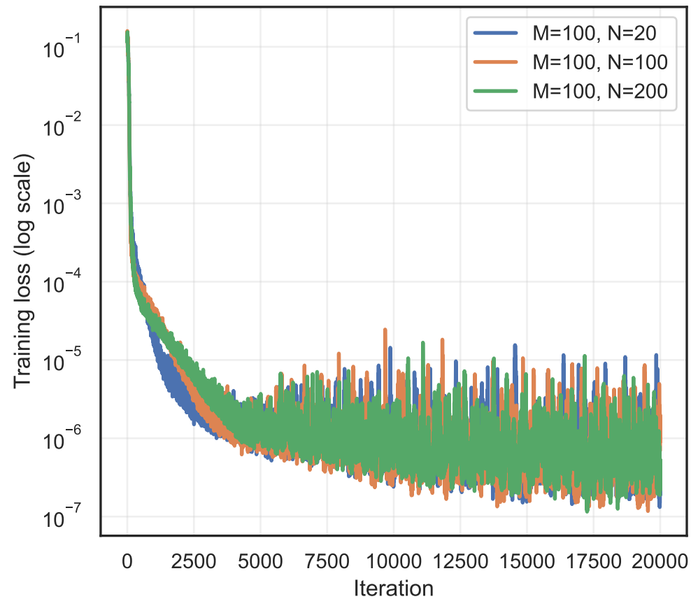
Loss decay for different (M, N)
