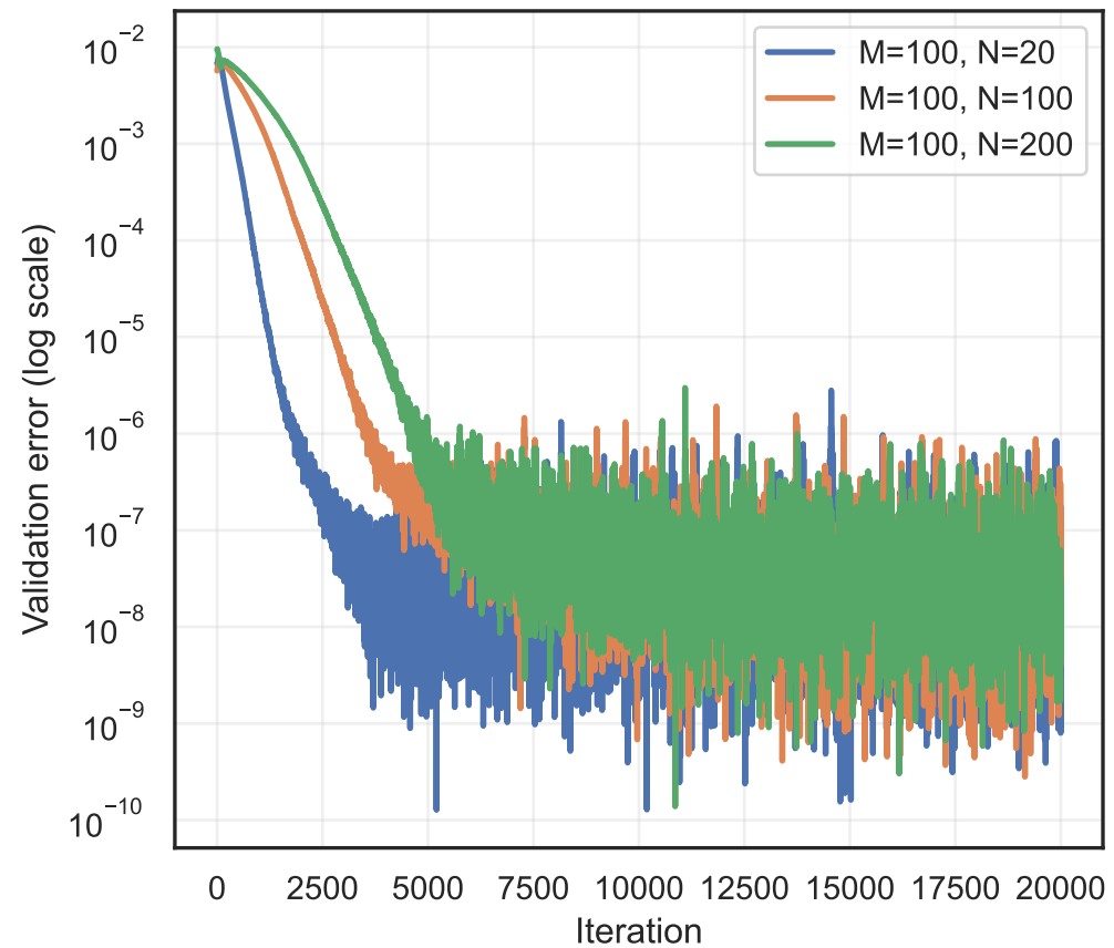
Y0 Error decay for different (M, N)
