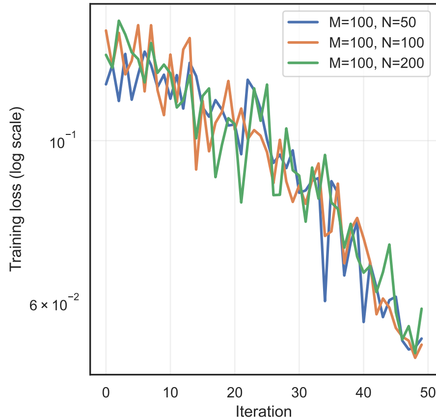
Loss decay for different (M, N)
