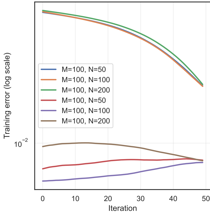
Error decay for different (M, N)
