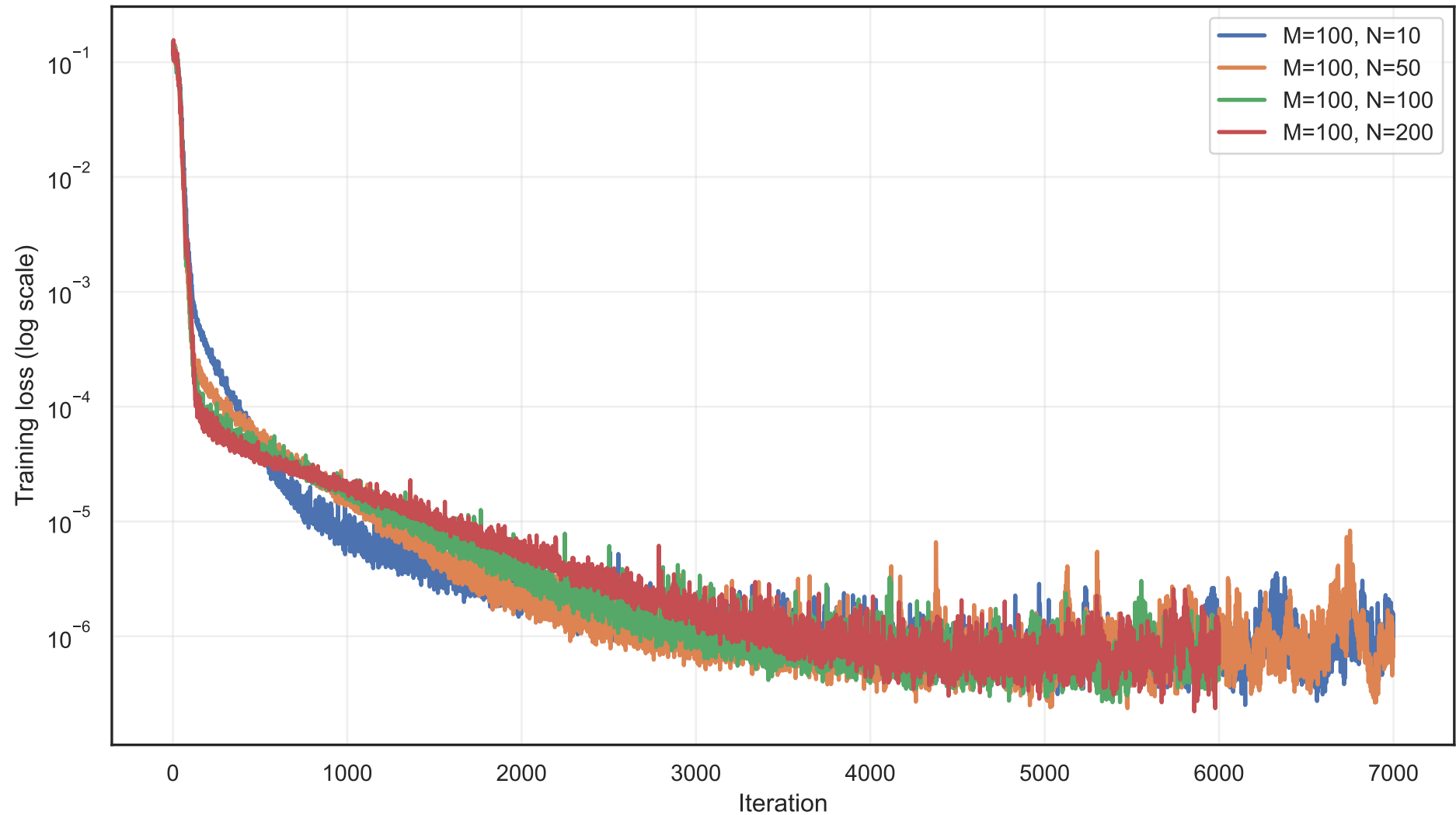
Training loss decay for different (M, N)
