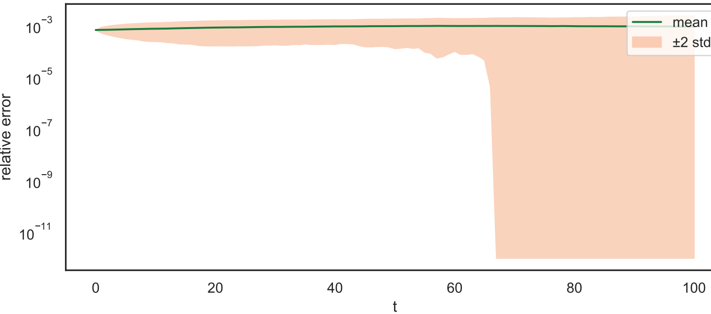
Portfolio strategy \theta^3
