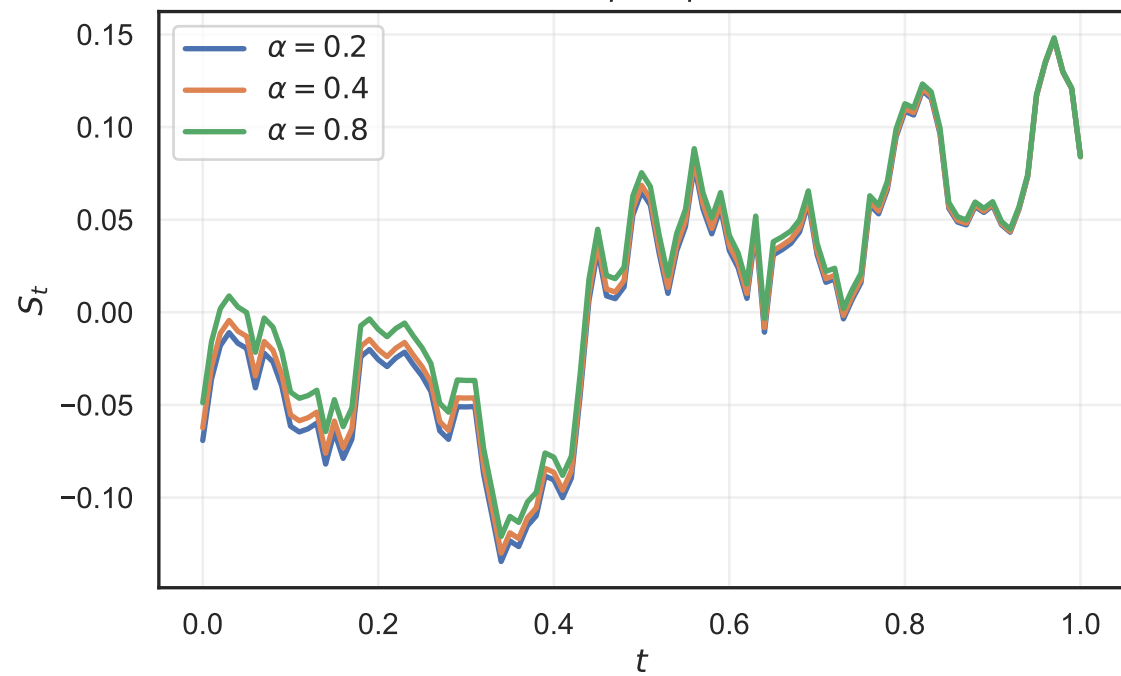
Stock price paths
