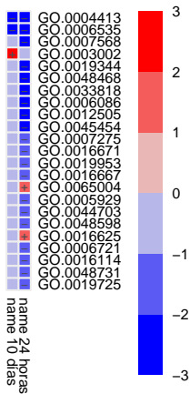
Significant associations (-\log(qval)*\text{sign}(coeff))
