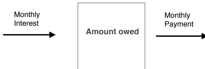
Figure 2.1: A compartmental diagram.
